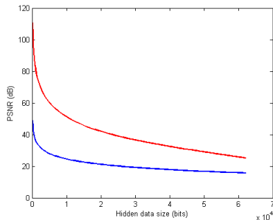
Figure 6. Curves of the average PSNR of the 18 decrypted video sequences versus the hidden data size.
