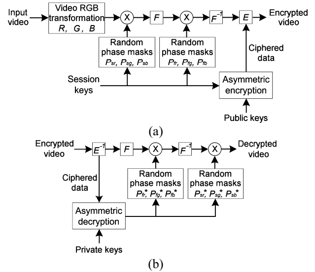
Figure 2. Schema of the proposed video cryptosystem. (a) Encryption, (b) Decryption (X: multiplication, E and E^{-1} : the embedding and decoding functions).
