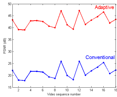
Figure 4. Curves of the PSNR values of the 18 decrypted video sequences ( QL=8 ; hidden data=19200 bits/frame).
