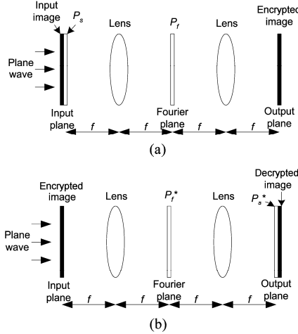
Figure 1. Schematic diagram for optical implementation of double random phase (a) encryption and (b) decryption ( f is focal length of the lens).
