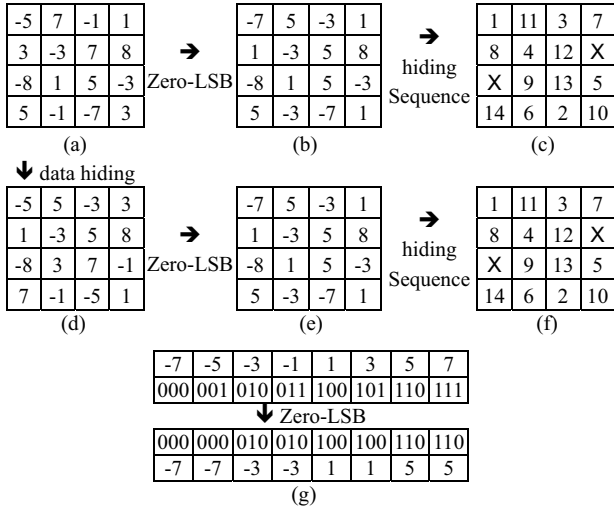
Figure 3. A simple example of data hiding and decoding ( QL=8 ; hidden data=11001110100011).
