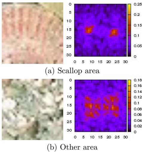
Figure 5: Object images and results of frequency analysis
