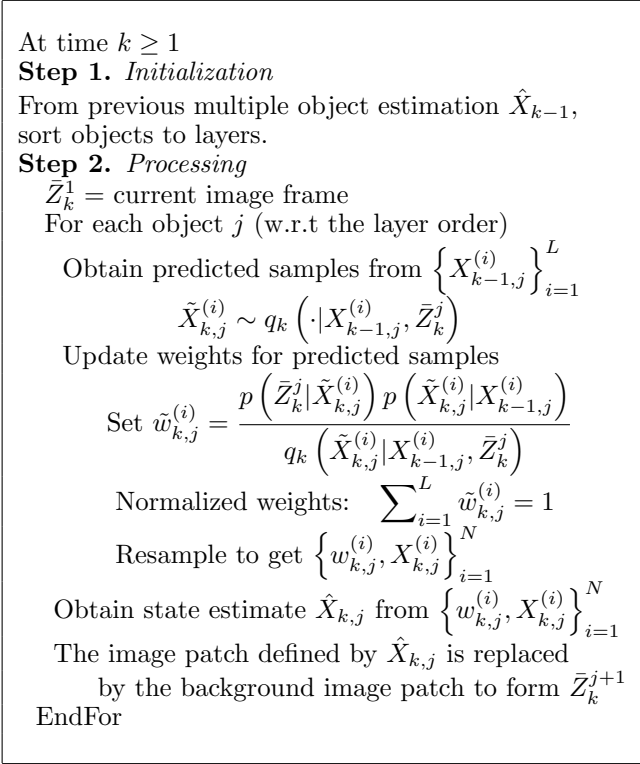
Figure 1. Sequential particle filter for multiple object tracking
