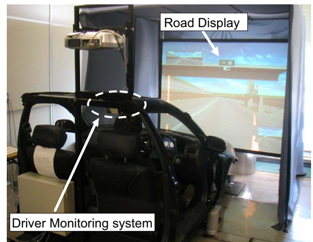
Fig.4 Driving Simulator
