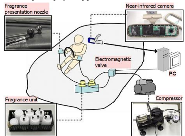
Figure1. Composition of fragrance presentation system
