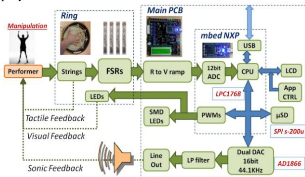
Figure 4. The Manipuller II Hardware Block Diagram
