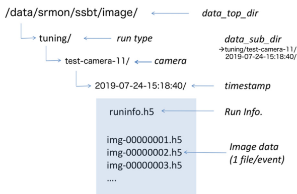
Figure 4: Directory structure of image file.
