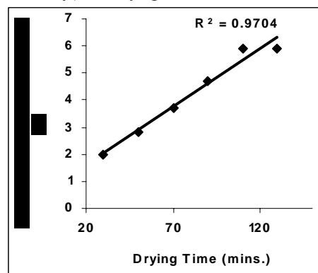
Figure 2: Variation of quantity of water evaporated (from Ukpore clay) with drying time
