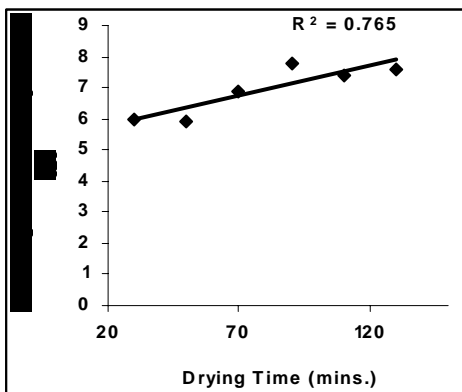
Figure 11: Variation of quantity of water evaporated (from Ukpör clay) with drying time
