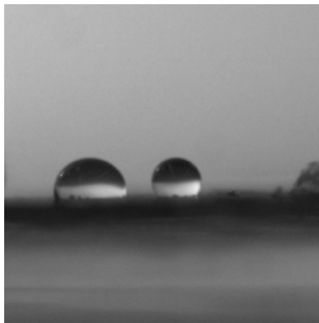
Figure 11. Photographs of water droplets on RuO 2 nanorods. The drop on the left is a dilute solution of H 2 SO 4 , while the drop on the right is DI water.
