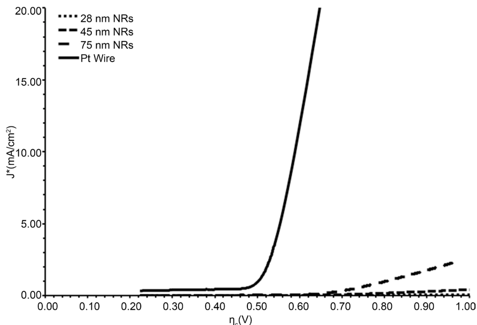
Figure 8. Cathode overvoltage of various electrodes including those coated with RuO 2 nanorods of varying width. A 3.5% aqueous solution of H 2 SO 4 was used as the electrolyte and a Pt wire used as the anode.
