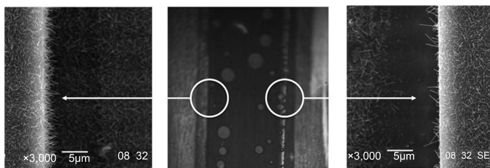
Figure 2. (Center) Top view photograph of bubble formation in the catalytic microchannel resulting from the decomposition of \text{H}_2\text{O}_2 monopropellant. The channel dimensions are 540 \mu\text{m} wide and 5 \mu\text{m} deep. (Left and Right) Magnified views of nanorod films along the sidewalls.
