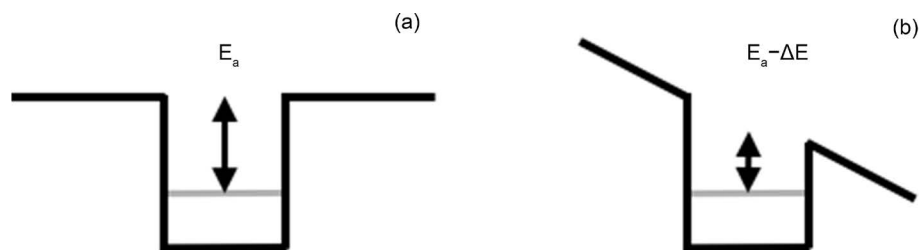
Figure 9. The simplified model of a particle in a finite, 1-D quantum well: (a) V = 0 and (b) V = finite magnitude.
