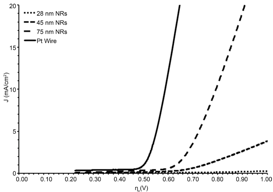
Figure 7. Cathode overvoltage of various electrodes including those coated with RuO 2 nanorods of varying width. A 3.5% aqueous solution of H 2 SO 4 was used as the electrolyte and a Pt wire used as the anode.
