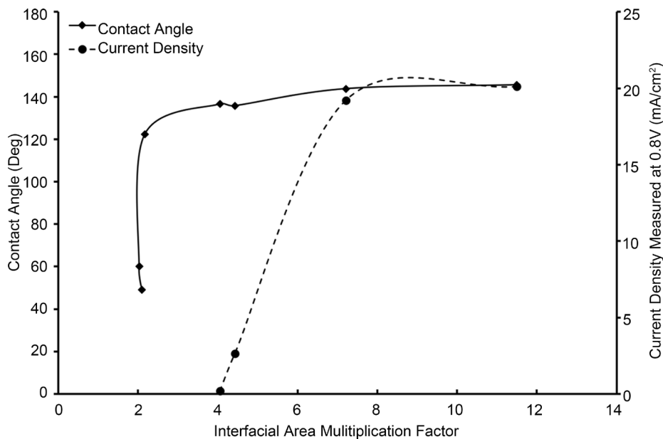
Figure 10. Contact angle and current density of RuO 2 nanorods grown on aluminized Si substrate. The electrolysis cell used a 3.5% aqueous solution of H 2 SO 4 as the electrolyte and a Pt wire used as the anode. The interfacial area multiplication factor is defined as the surface area of the nanorods times their density.
