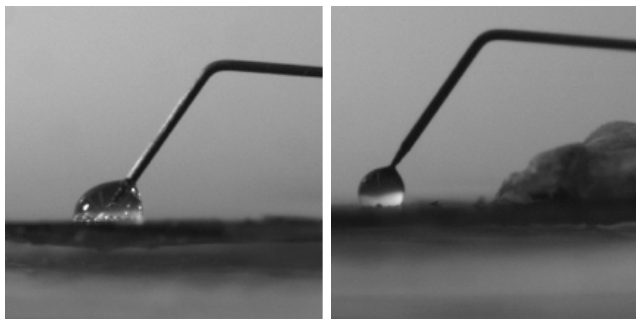
Figure 12. Photographs of electrically charged water droplets on RuO 2 nanorods. (Left) The drop is a dilute solution of H 2 SO 4 ; (Right) The drop is DI water.
