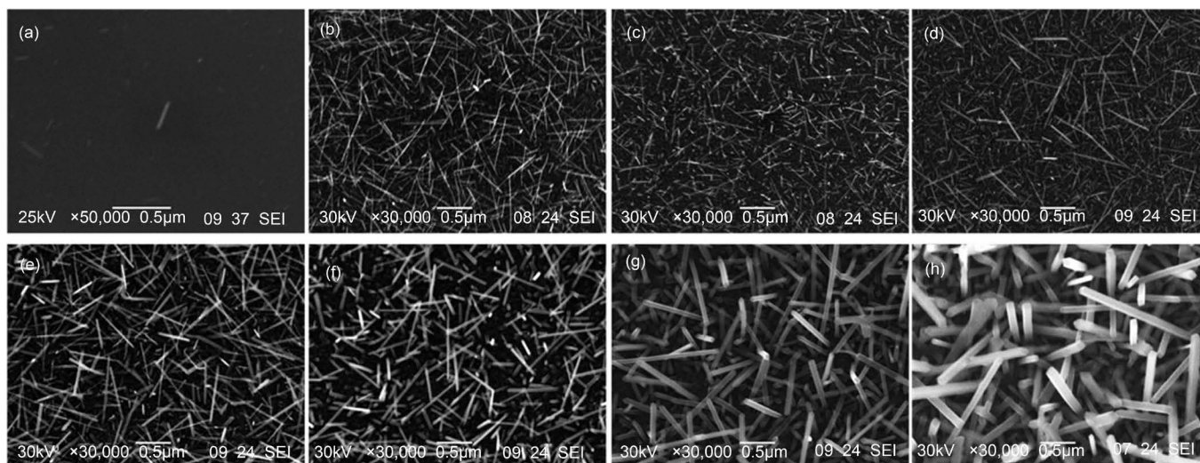
Figure 3. SEM images of RuO 2 nanorods grown on aluminized Si substrate. The scale bar in all images is 0.5 μm. Nanorod length/width/density are: (a) 0.2 μm/18.6 nm/0.2 μm -2 , (b) 0.7 μm/21.0 nm/18.7 μm -2 , (c) 0.7 μm/19.0 nm/19.3 μm -2 , (d) 0.8 μm/22.0 nm/16.6 μm -2 , (e) 1.0 μm/29.0 nm/26.3 μm -2 , (f) 0.9 μm/34.0 nm/28.0 μm -2 , (g) 1.3 μm/66.0 nm/18.1 μm -2 , (h) 1.6 μm/100.0 nm/16.4 μm -2 .
