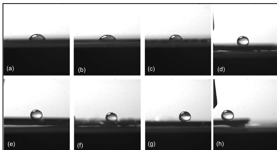
Figure 4. Photographs of DI water droplet on RuO 2 nanorods. The total nanorod area (defined as the surface area of the nanorods times their density) are (a) 1.0 μm 2 /μm 2 , (b) 2.1 μm 2 /μm 2 , (c) 2.0 μm 2 /μm 2 , (d) 2.2 μm 2 /μm 2 , (e) 4.1 μm 2 /μm 2 , (f) 4.4 μm 2 /μm 2 , (g) 7.2 μm 2 /μm 2 , and (h) 11.5 μm 2 /μm 2 .
