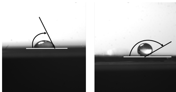
Figure 5. Definition of contact angle measurement for (left) a wetting sample and (right) a non-wetting sample.
