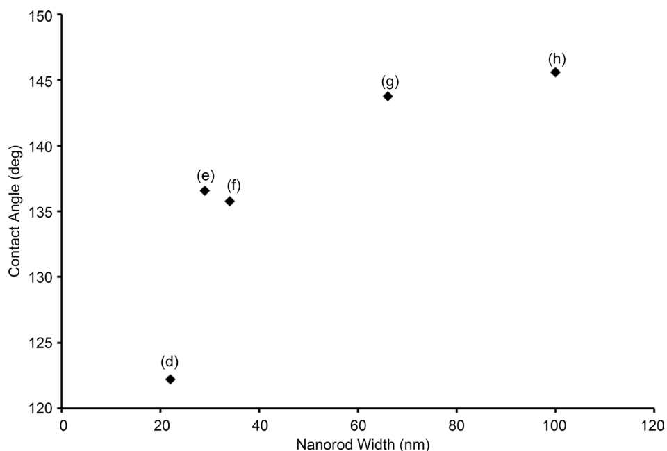
Figure 6. Contact angle of droplets on RuO 2 nanorods. The data labels correspond to the images shown in Figure 3 and Figure 4 .
