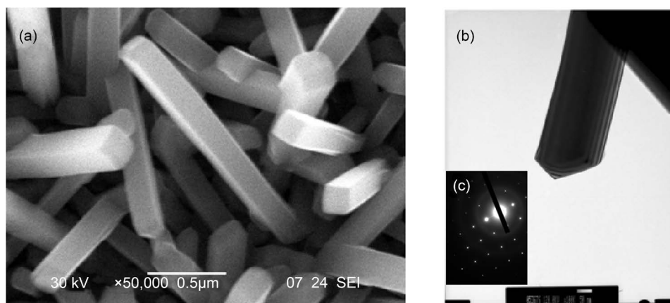
Figure 1. (a) SEM image of square RuO 2 nanorods grown on a Si substrate. (b) TEM scan of an individual nanorod, showing an atomically sharp pyramid tip. (c) Diffraction pattern indicates crystallinity.
