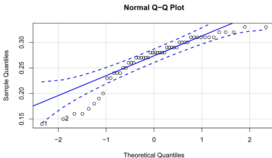
Figure 2. QQ plot for testing normality.
