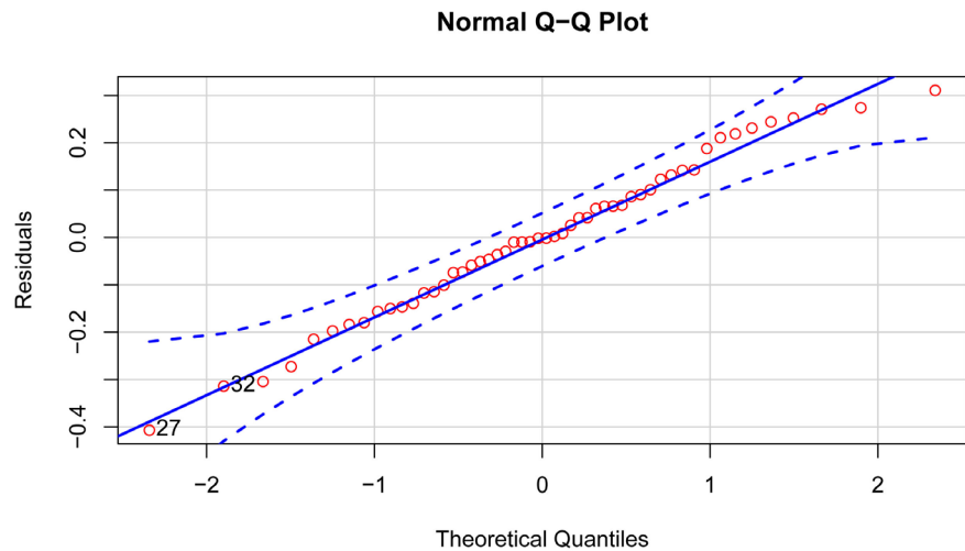
Figure 7. QQ plot for testing the normality of residuals with 95% confidence limits.
