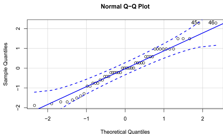
Figure 5. QQ plot for testing the normality of \text{TCO}_2 .
