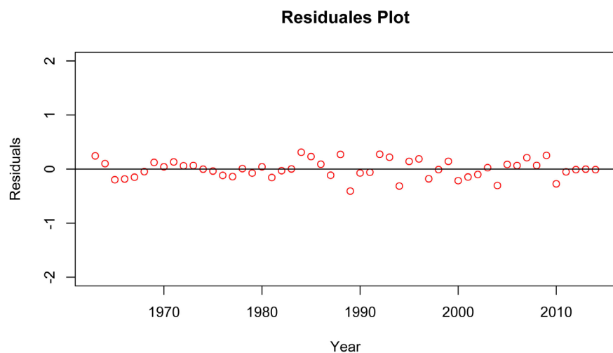
Figure 8. Scatter plot for testing the pattern of residuals.
