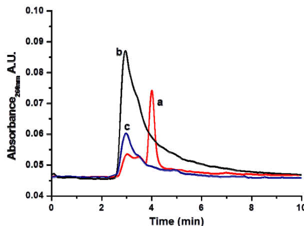
Figure 3. Chromatograms of 1.0 \text{ g} of soil contaminated with an aqueous solution of 10 \text{ mg}\cdot\text{L}^{-1} atrazine, in its extraction it was used (a) Triton X-114, (b) SDS and (c) CTAB, all at CMC. Flow rate: 1.0 \text{ mL}\cdot\text{min}^{-1} , \lambda = 260 \text{ nm} , in an agilent eclipse \text{C}_{18} PAH column. Mobile phase \text{CH}_3\text{OH}/1 \times 10^{-3} phosphate buffer, pH 2.6/ \text{CH}_3\text{CN} 60:30:10 (v/v).
