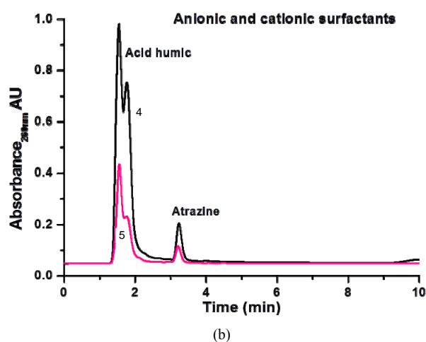
Figure 4. Chromatograms of extraction from 1.0 g clean soil contaminated with 10 mg·L -1 atrazine by using 3 mL of aqueous extractant solution at CMC. (a) non ionic extraction: (1) X-114, (2) Triton X-100 and (3) TritonX-405; (b) ionic extraction: (4) anionic SDS, (5) cationic CTAB at CMC. Flow rate: 0.4 ml/min., \lambda = 260 nm, agilent eclipse C 18 PAH column. Mobile phase CH 3 OH/1 × 10 -3 M. Phosphate buffer, pH 3.2/CH 3 CN 55:30:15 (v/v).
