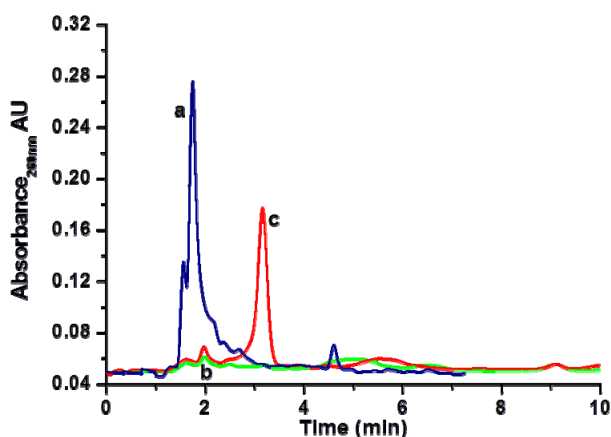
Figure 2. Chromatograms for extracts obtained from: (a) 5 \text{ mg}\cdot\text{L}^{-1} humic acid/ \text{CH}_3\text{CN} ; (b) 1.0 \text{ g} clean soil/ \text{CH}_3\text{CN} ; (c) 1.0 \text{ g} soil previously contaminated with 10 \text{ mg}\cdot\text{L}^{-1} atrazine/ \text{CH}_3\text{CN} , and experimental detection conditions: flow rate: 0.4 \text{ mL}\cdot\text{min}^{-1} , \lambda = 260 \text{ nm} , agilent eclipse \text{C}_{18} PAH column. Mobile phase \text{CH}_3\text{OH}/1 \times 10^{-3} , phosphate buffer, pH 3.2/ \text{CH}_3\text{CN} 60:30:10 (v/v).
