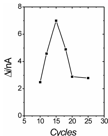
Figure 2. Effect of the polymerization cycle number on the response current of the Au/POAP/CNT/GOD electrode. Steady-state currents are measured at 0.75 V (SCE) in 1/15 M phosphate buffer solution (pH 7) containing 2 mM glucose ( n = 3 ) [30].
