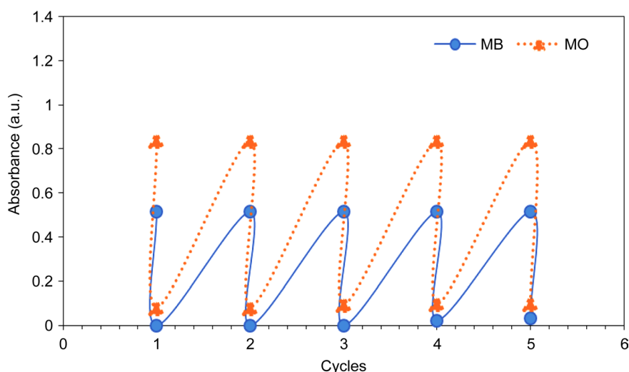
Figure 11. Five cycles of photocatalytic degradation of MB and MO using the core-shell nanospheres.
