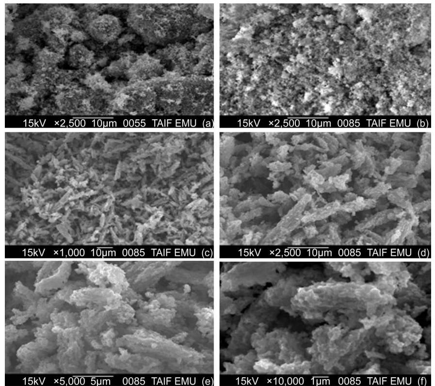
Figure 3. SEM images of \text{Fe}_3\text{O}_4 (a), \text{Fe}_3\text{O}_4/\text{SiO}_2 (b), and \text{Fe}_3\text{O}_4/\text{SiO}_2/\text{TiO}_2 nanocomposites (c)-(f).
