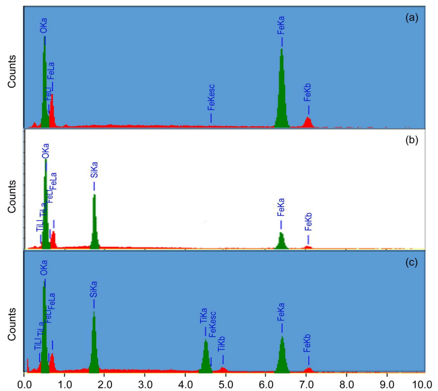
Figure 4. EDAX spectra of (a) \text{Fe}_3\text{O}_4 , (b) \text{Fe}_3\text{O}_4/\text{SiO}_2 , and (c) \text{Fe}_3\text{O}_4/\text{SiO}_2/\text{TiO}_2 nanocomposites.
