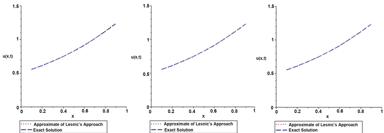
Figure 11. The exact solution and the approximate solution of Lesnic’s approach for \varphi_3, \varphi_5, \varphi_{10} at t = 0.5 .
