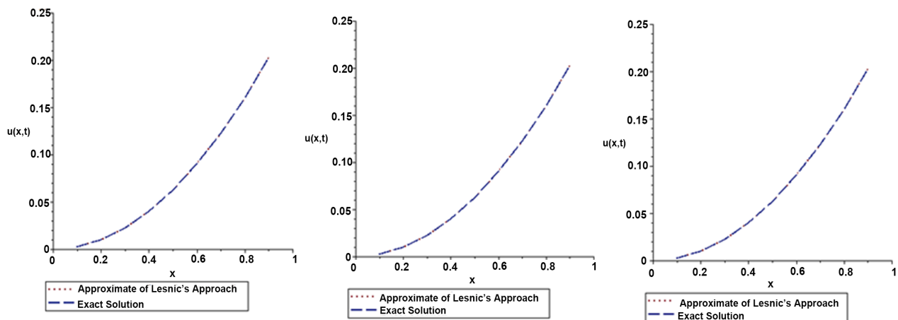
Figure 9. The exact solution and the approximate solution of Lesnic’s approach for \varphi_3, \varphi_5, \varphi_{10} at t = 0.5 .
