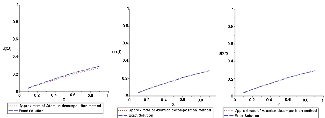
Figure 2. The exact solution and the approximate solution using ADM for \varphi_3, \varphi_5, \varphi_{10} at t = 1.0 and 0 \leq x \leq 1 .
