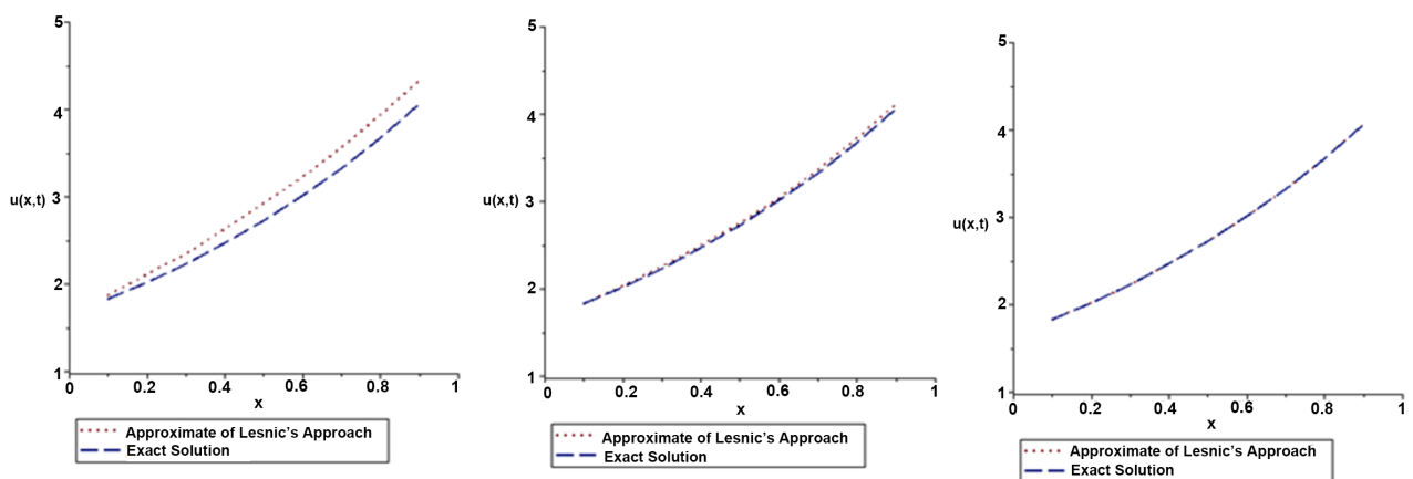
Figure 5. The exact solution and the approximate solution of Lesnic’s approach for \varphi_3, \varphi_5, \varphi_{10} at t = 0.5 .
