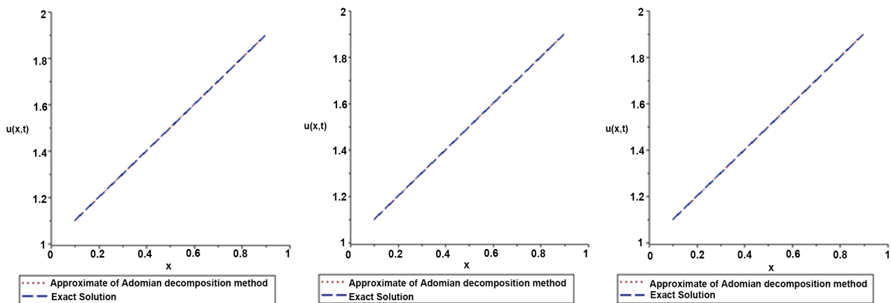
Figure 4. The exact solution and the approximate solution using ADM for \varphi_3, \varphi_5, \varphi_{10} at t = 1.0 .
