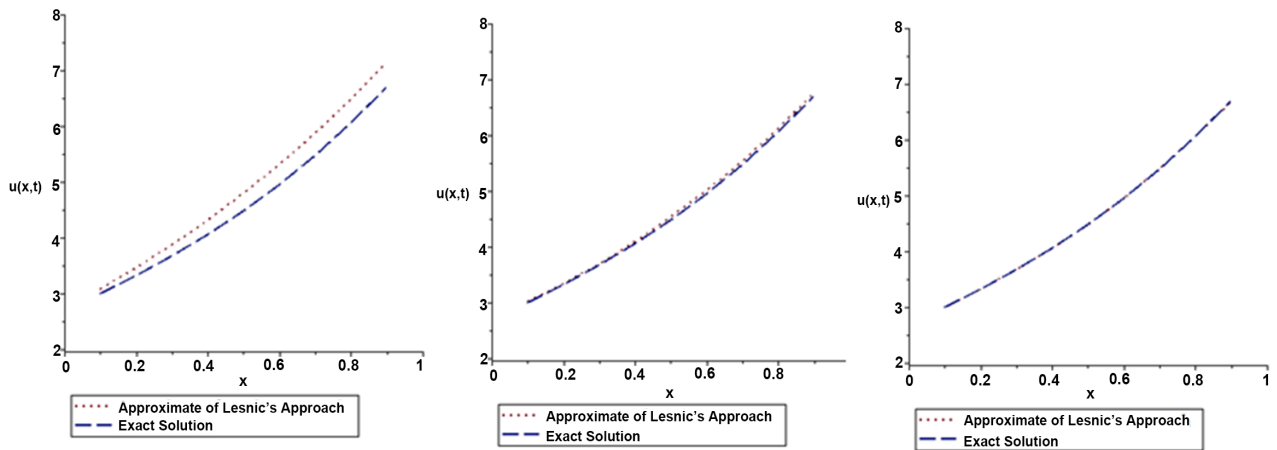
Figure 6. The exact solution and the approximate solution of Lesnic's approach for \varphi_3, \varphi_5, \varphi_{10} at t = 1.0 .
