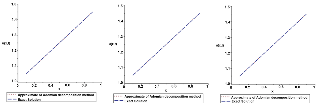
Figure 3. The exact solution and the approximate solution using ADM for \varphi_3, \varphi_5, \varphi_{10} at t = 0.5 .
