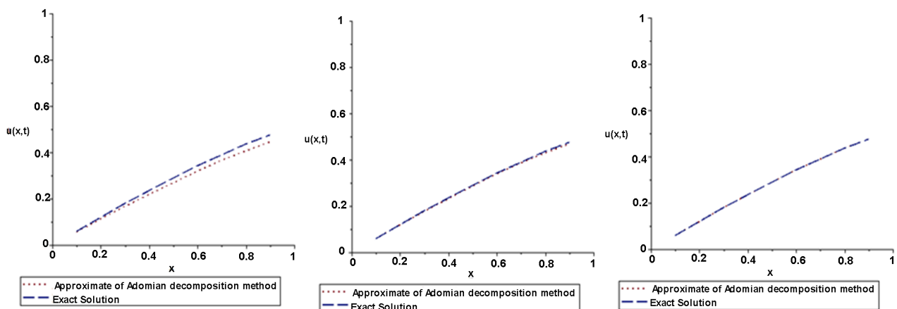
Figure 1. The exact solution and the approximate solution using ADM for \varphi_3, \varphi_5, \varphi_{10} at t = 0.5 and 0 \leq x \leq 1 .
