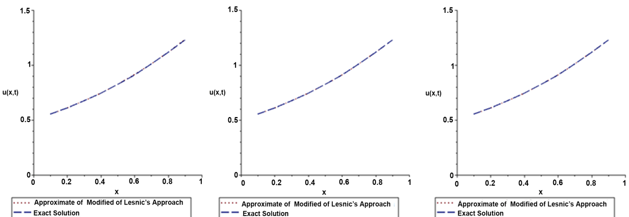
Figure 12. The exact solution and the approximate solution of Modified of Lesnic’s approach for \varphi_3, \varphi_5, \varphi_{10} at t = 0.5 .
