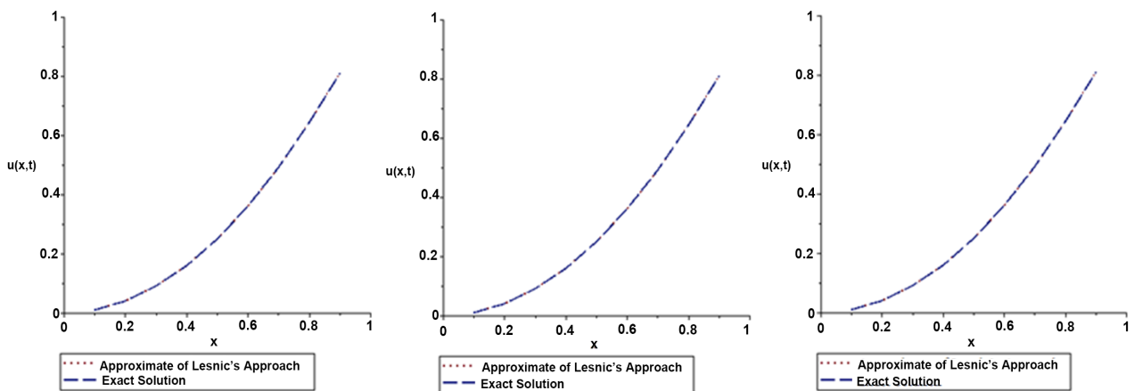
Figure 10. The exact solution and the approximate solution of Lesnic’s approach for \varphi_3, \varphi_5, \varphi_{10} at t = 1.0 .
