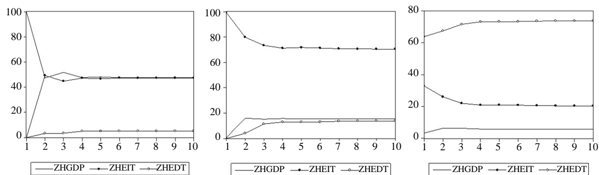
Figure 4. Variance decomposition of ZHGDP, ZHEIT, ZHEDT.
