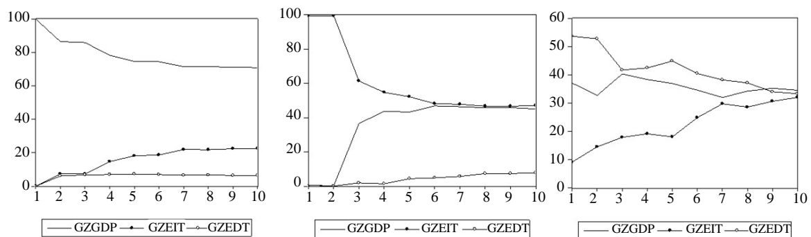
Figure 2. Variance decomposition of GZGDP, GZEIT, GZEDT.
