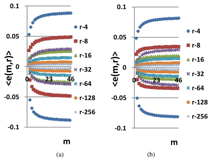
Figure 12. Distributions of Hölder's averages \langle e(m, r) \rangle with different number m for fluctuations of entropy e(r) near homeostasis for a good health man in real time, during one year; initial histograms for Figure 12(a) and 12(b) are presented in Figures 6 and 7(a) for yellow and green points; distribution of Hölder's averages for red quadrature points in Figure 6 presented in Figure 10(b) ; upper and lower branches correspond to the even m = 2, 4, 6, \dots and odd m = 1, 3, 5, \dots
