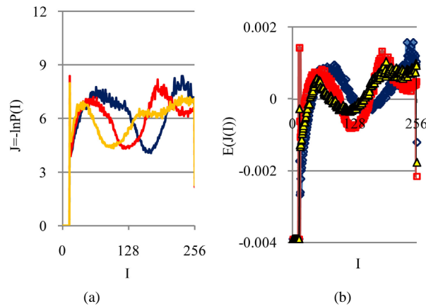
Figure 2. (a) Logarithmic dependence \text{LnP}(I) for frequency of flashes P(I) on their intensity I(r = 256) ; The area under the initial histograms of P(I) normalized to unit; Original histograms for P(I) shown in Figure 1 ; (b) Normalized distributions of information entropy E(J(I)) in the dependence on fluorescence intensity I(r = 256) ; rhombuses correspond to bronchial asthma. Total number of flashes is N_0 = 76\,623 ; squares correspond to the healthy donor, N_0 = 40\,109 ; cross correspond to the oncology disease. Common number of flashes is N_0 = 40\,752 .
