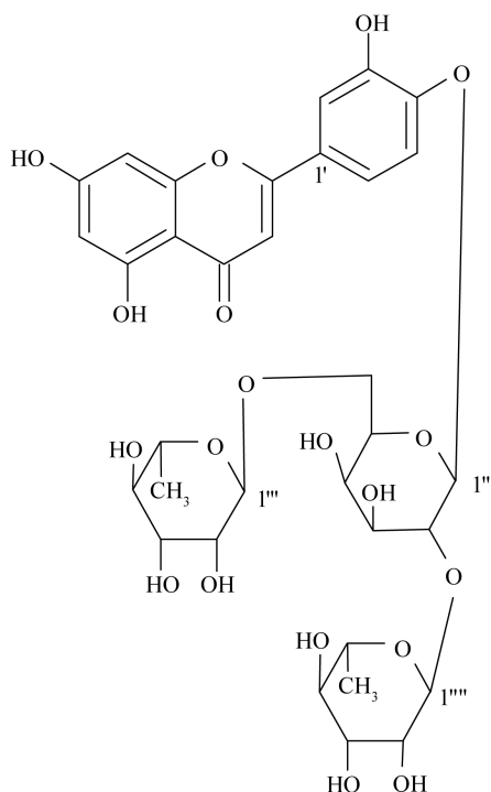
Luteolin-4'-O-[\mathbf{\alpha}-L-rhamnopyranosyl-(1 \rightarrow 2)-{\mathbf{\alpha}-L-rhamnopyranosyl-(1 \rightarrow 6)}-\mathbf{\beta}-D-glycopyranoside].
