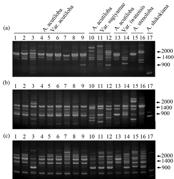
Figure 1. RAPD profiles generated by OPA-16 (a), OPD-3 (b) and OPD-15 (c) primers. Lanes 1 - 9: A. acutiloba var. acutiloba (TG, TK, TY, TH, TC, YB, YM, OT, OC; refer to Table 1 for codes), lanes 10 - 12: A. acutiloba var. sugiyamae (HA, HB, HC), lanes 13 and 14: A. acutiloba var. iwatensis (MM, MY), lane 15: A. stenoloba (LH), lane 16: A. lanceolata (LT), lane 17: A. shikokiana (IM).
