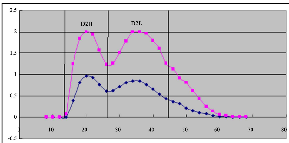
Figure 3. Purification of D2 by gel permeation chromatography.
