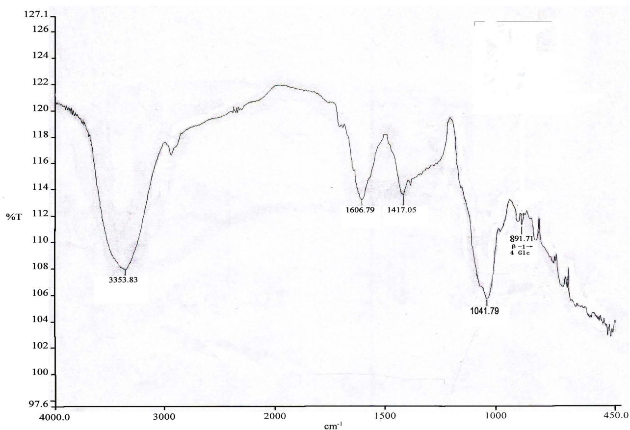
Figure 4. IR spectrum of D2.
