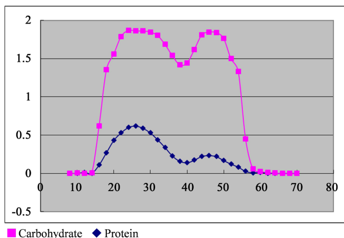
Figure 1. Gel permeation chromatography on Sephadex G-150 of Sample P.
