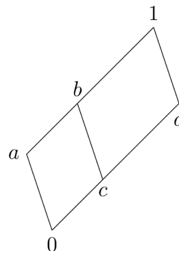
Diagram 8. A closed join sub-semilattice.
