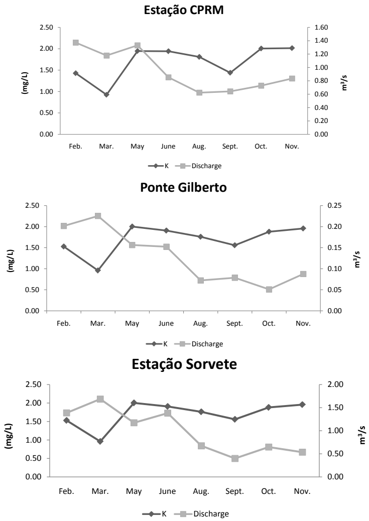
Figure 8. Variation of potassium concentration according to discharge.
