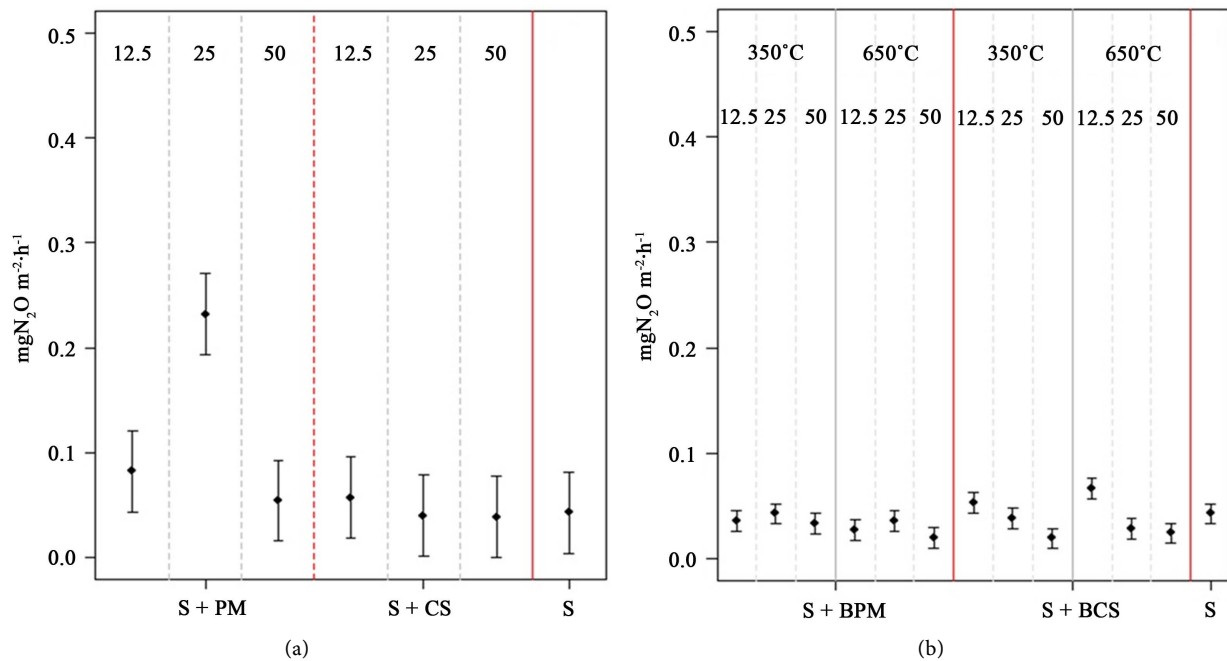
Figure 3. Emission of \text{N}_2\text{O} from a tropical sandy soil (S) amended with a) raw materials: poultry manure (S + PM) and sugar cane straw (S + CS); and b) biochars: biochar poultry manure (S + BPM) and biochar of sugar cane straw (S + BCS).
