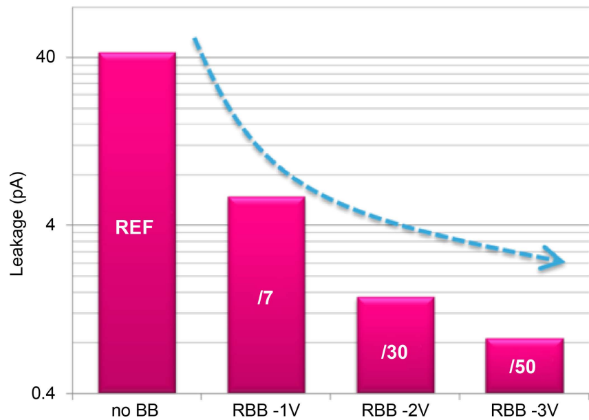
Figure 12. RBB impacts on leakage current [16].
