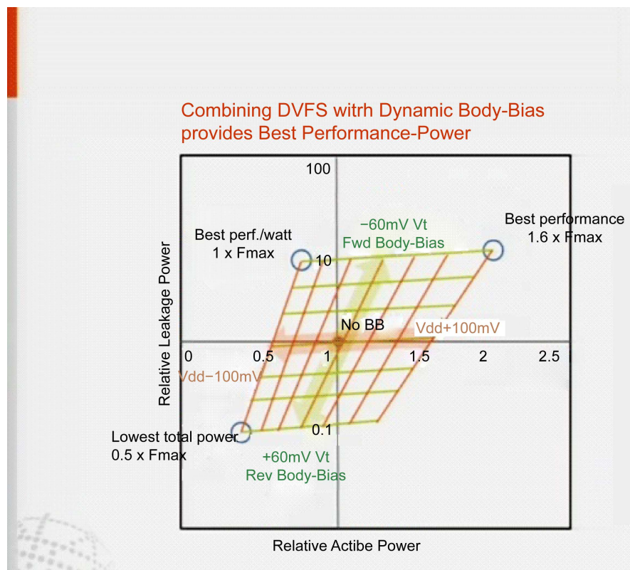
Figure 11. Combining DVFS with body Bias [17].
