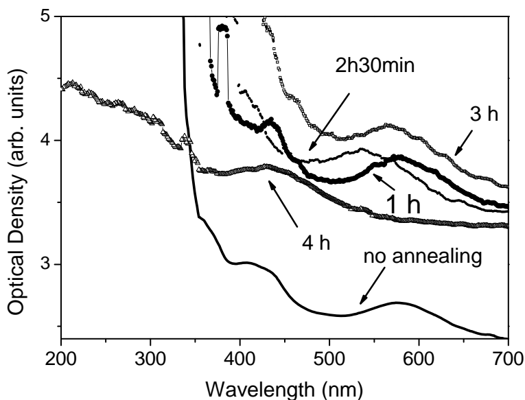
Figure 2. Optical absorption spectra of natural alexandrite as function of consecutive annealing
