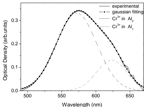
Figure 3. Decomposition of band A of optical absorption spectra in two Gaussian curves for synthetic alexandrite
