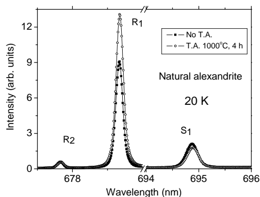
Figure 4. Photoluminescence spectra of natural alexandrite, measured at 20 K, before any thermal annealing and after the final annealing at 1000°C, 4 hour
