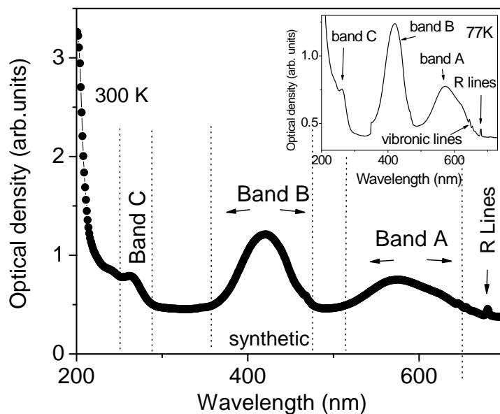
Figure 1. Optical absorption spectra of synthetic alexandrite samples, measured at room temperature (300K). Inset-optical absorption spectra of synthetic alexandrite, measured at liquid nitrogen temperature (77K).
