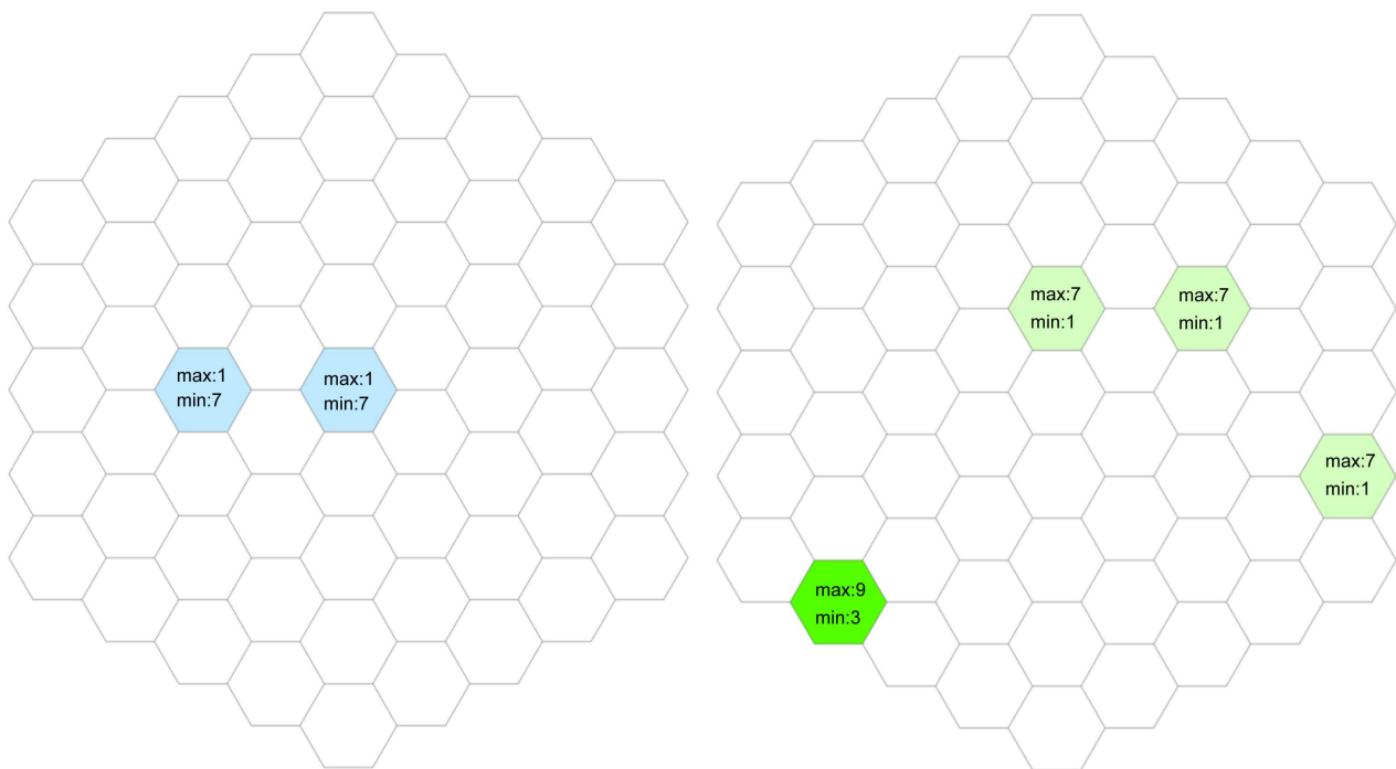
Figure 8. Nets corresponding to a region with two cells containing hydro power plants (left) and four cells containing wind turbines (right).
