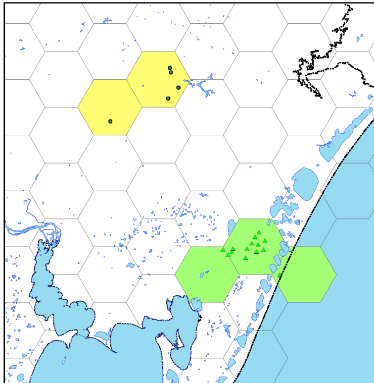
Figure 12. A network with 500 km 2 cells assembled to evaluate spatial complementarity in the region of the northern coast of the State of Rio Grande do Sul.
