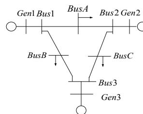
Figure 2. Electric diagram of IEEE 9-Bus system.
