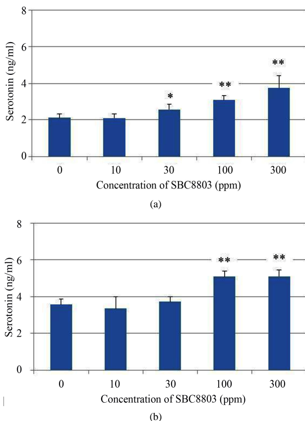
Figure 1. Influence of concentration of Lactobacillus brevis SBC8803 on 5-HT release from rat endocrine RIN-14B cells. The results obtained after incubation for 30 min are shown in (a). * P < 0.05 for 0 ppm vs. 30 ppm; ** P < 0.01 for 0 ppm vs. 100 ppm and 300 ppm. The results obtained after incubation for 60 min are shown in (b). ** P < 0.01 for 0 ppm vs. 100 ppm and 300 ppm. Results are represented as mean \pm SD ( n = 4 ).
