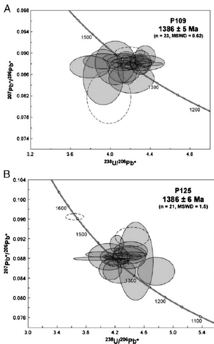
Figure 6. Analytical data for zircons, obtained in Curtin University, Australia (Puchkov et al., 2013). A. U-Pb analytical data for zircons from sample P109: Dunansungan rhyolite, Mashak Formation. Dashed ellipses indicate analyses not included in the calculation of the weighted mean ^{207}\text{Pb}^*/^{206}\text{Pb}^* date, which is quoted with 95% confidence limits. B. U-Pb analytical data for zircons from sample P125: Shatak dacite-rhyolite, Mashak Formation. Dashed ellipses indicate analyses not included in the calculation of the weighted mean ^{207}\text{Pb}^*/^{206}\text{Pb}^* date, which is quoted with 95% confidence limits.
