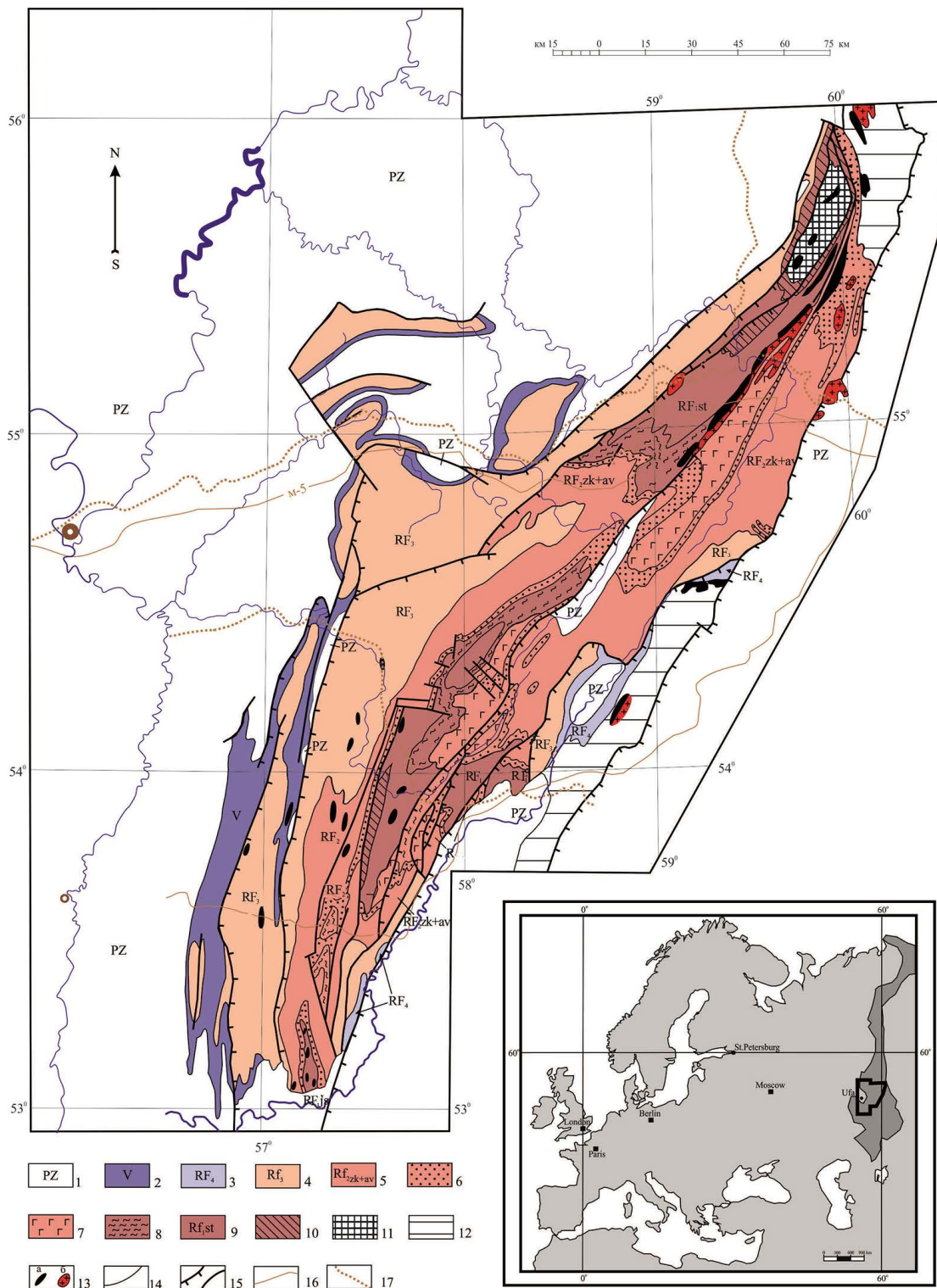
Figure 1. Geological map of the Bashkirian anticlinorium After Geological Survey map... 2002, strongly modified. 1—Paleozoic, 2—Vendian, 3—Uppermost Riphean, 4—Upper Riphean, 5—Middle Riphean, Zigazino-Komarov and Avzyan Formations, 6—Zigalga Formation of the Middle Riphean, 7—Mashak Formation of the Middle Riphean, 8 - 10—Lower Riphean: 8—Bakal and Jusha Formation, 9—Satka and Suran Formations, 10—Ai and Bolsheiner Formations. 11—Archean-Paleoproterozoic Taratash complex. 12—Upper Riphean Northern Uraltau complex. Intrusions: 13a—mafic, 13b—granitic, 14—stratigraphic contacts, 15—tectonic contacts: thrusts and normal faults, 16—highways, 17—railroads.
