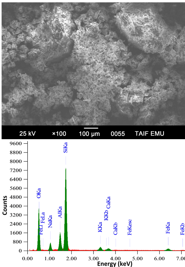
Figure 5. EDS spectrum (down) and corresponding SEM image (up) for most radioactive anomalous granite AG2.
