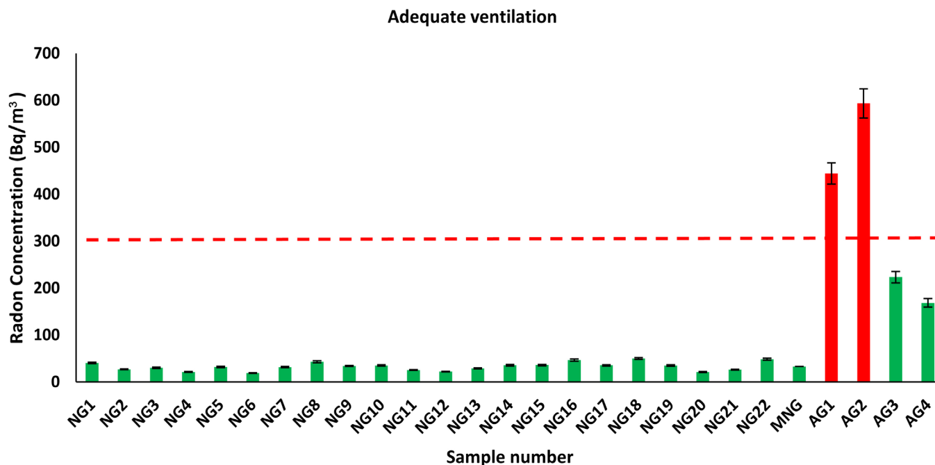
Figure 3. Radon concentration for adequately ventilated room ( \lambda_v = 0.5 \text{ h}^{-1} ) (Reference level in broken line).
