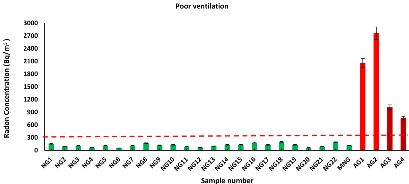
Figure 4. Radon concentration for poorly ventilated room ( \lambda_v = 0.1 \text{ h}^{-1} ) (Reference level in broken line).
