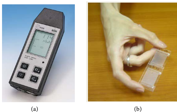
Figure 1. Measurements of natural photon and gamma radiation dose were performed with the Radiameter in the open atmosphere 1 m above the ground. The neutron dosimeter consisted of CR-39 track detector ( 2 \times 3 \text{ cm}^2 ; Intercast Europe Company of Parma, Italy) and boron foil BN-1 or 10 B converter (Kodak-Pathe, France).
