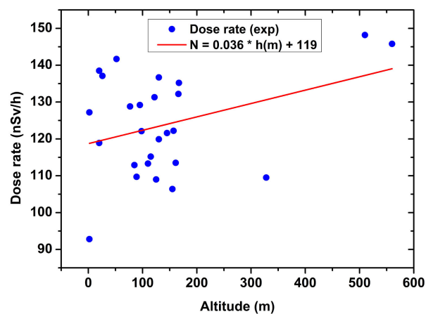
Figure 3. Neutron dose rate N versus altitude h of the MS (experimental data + linear regression with Microsoft Excel).
