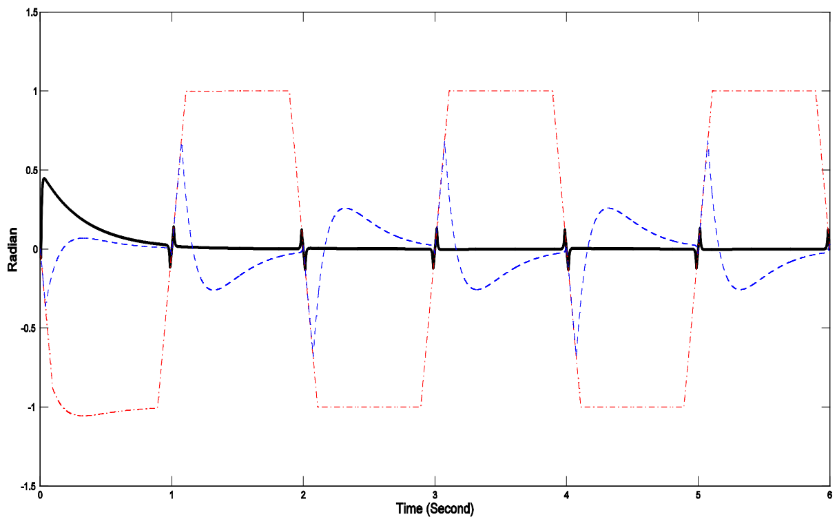
Figure 4. The output tracking error y_o (solid) for the system under RAODI vs. the tracking error of the system under a PD-controller (red-dashed). The dashed blue line reflects the output tracking error for the system without the use of inverse deadzone modifier.
