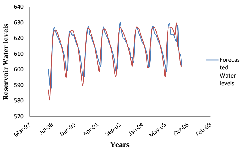
Figure 3. Forecast of water levels in the Warna reservoir (red line is the observed water level, blue line is water level forecast).
