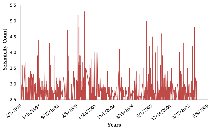
Figure 1. Time series of earthquake counts from 1996-2008.
