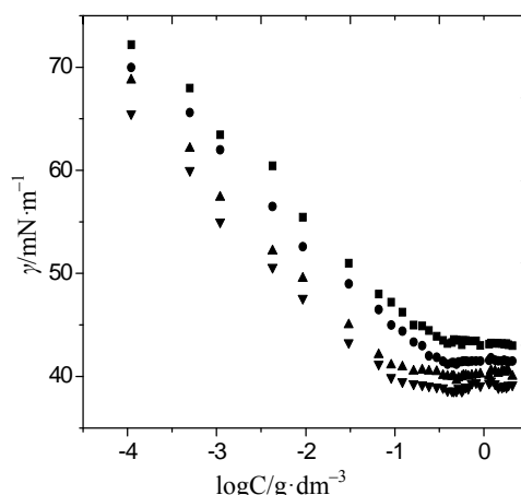
Figure 1. Typical Plots of surface tension ( \gamma ) as a function of logarithmic concentration ( \log C ) for aqueous solutions of E_{58}B_{11} at (■) 20°C, (●) 30°C, (▲) 40°C and (▼) 50°C.
