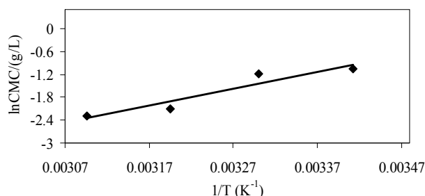
Figure 3. Typical plot of logarithm of CMC (lnCMC) versus inverse of temperature for aqueous solutions of E 58 B 11 .
