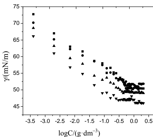
Figure 2. Typical Plots of surface tension ( \gamma ) as a function of logarithmic concentration ( \log C ) for aqueous solutions of E_{56}B_{19} at (■) 20°C, (●) 30°C, (▲) 40°C and (▼) 50°C.
