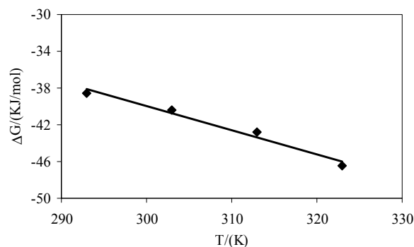
Figure 4. Typical plot of Gibbs free energy of adsorption versus temperature for aqueous solutions of E 58 B 11 .
