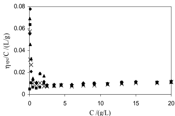
Figure 7. Typical plots of concentration dependence of reduced viscosity for aqueous solutions of E_{56}B_{19} at temperatures ( \blacksquare ) 20, ( \blacklozenge ) 30, ( \blacktriangle ) 40, and ( \times ) 50°C.
