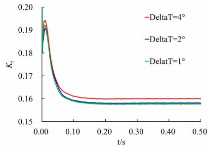
Figure 5. Time histories of K_t with different time step schemes.
