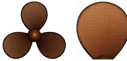
Figure 4. Distribution of grids (left: propeller grid; right: blade grid).
