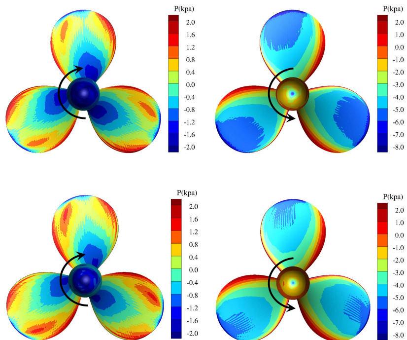
Figure 7. Pressure distribution on blades (top: restricted channel; bottom: open water).
