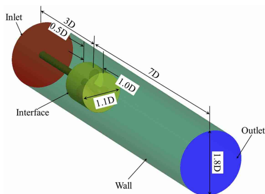
Figure 3. Domain and boundary conditions.
