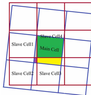
Figure 2. Arbitrary mesh interface.
