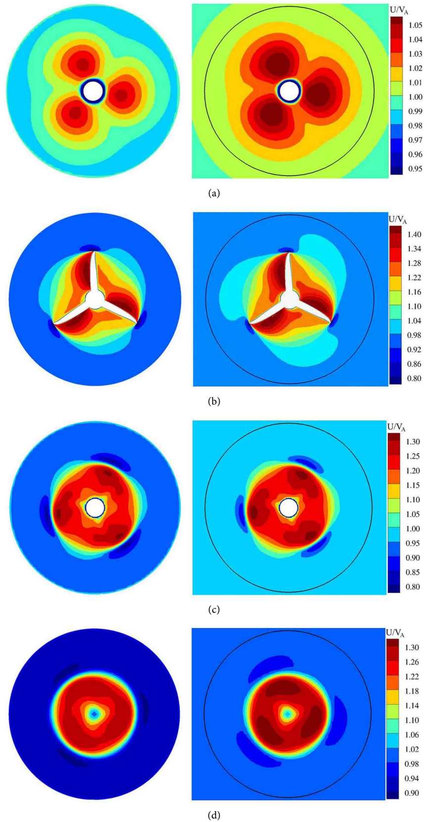
Figure 10. Axial velocity at different cutting planes (a: x/D = -0.30 ; b: x/D = 0.0 ; c: x/D = 0.25 ; d: x/D = 1.0 ; left: restricted channel; right: open water).
