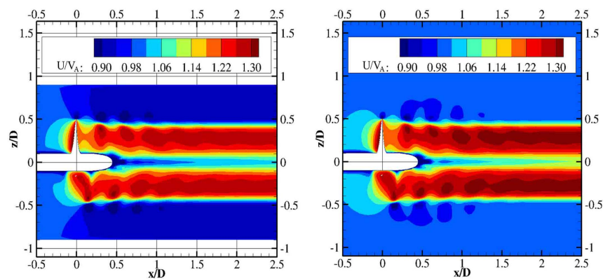
Figure 9. Axial velocity distribution (left: restricted channel; right: open water).
