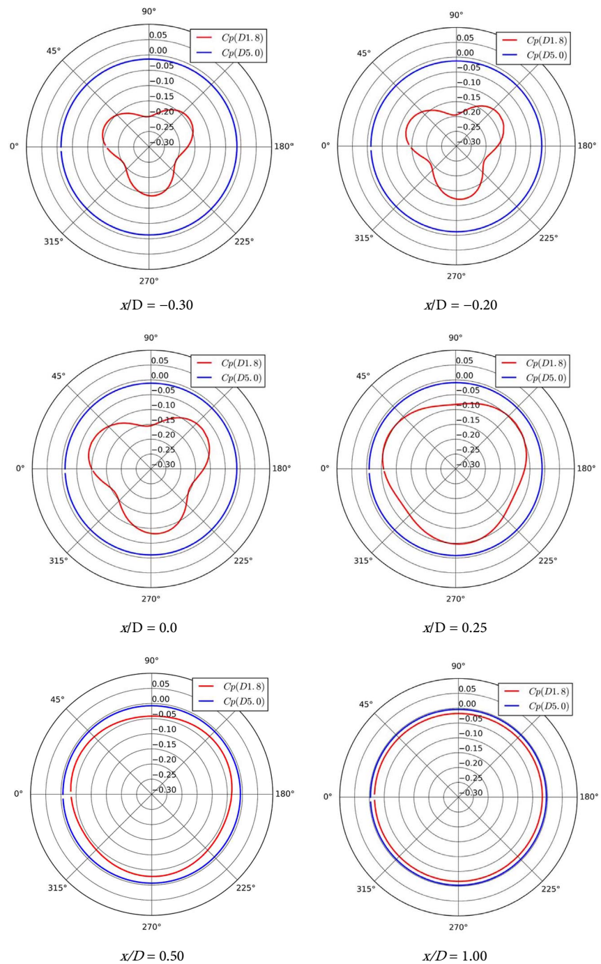
Figure 8. Pressure coefficient distribution on the wall of tunnel (Red: restricted channel; Blue: open water).
