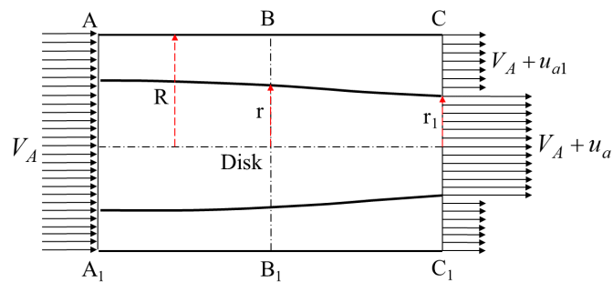
Figure 11. Hydrodynamic model of ideal thruster.
