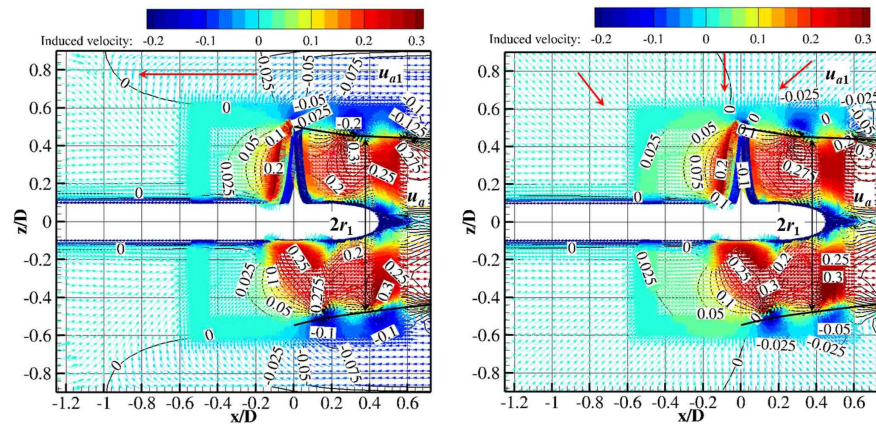
Figure 12. Induced velocity vector distribution (Left: restricted channel; right: open water).
