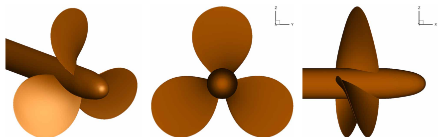
Figure 1. Geometry of DTMB 4119 propeller (left: 3D view; middle: front view; right: side view).
