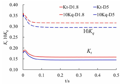
Figure 6. Time histories of thrust and torque coefficient at J = 0.833 .
