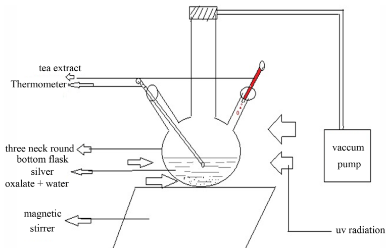
Figure 1. Experimental set-up.
