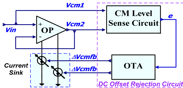
Figure 4. The principle of the DC offset rejection technique.
