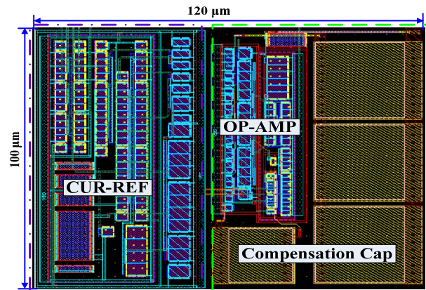
Figure 5. Layout view of the integrated CMOS amplifier.
