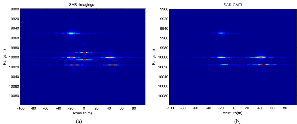
Figure 4. Motion modulation scatter-wave Jamming of moving jammer 2 and scene images simulation images ( \tau_s = 0.1\mu s ). (a) Image; (b) GMTI.
