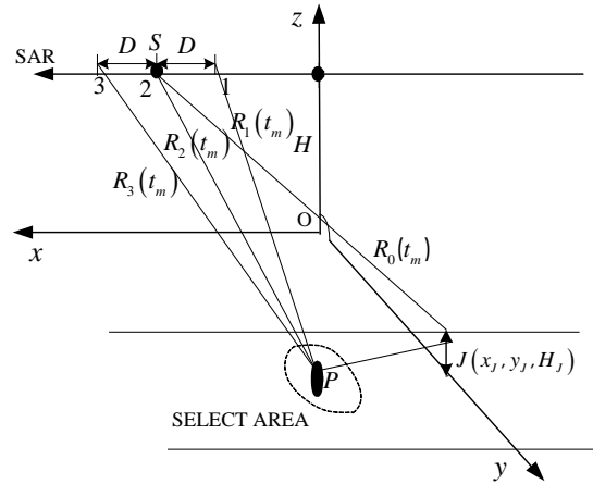
Figure 1. The jamming layout.
