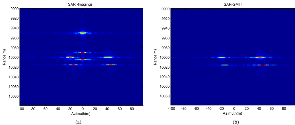
Figure 3. Motion modulation scatter-wave jamming of stationary jammer1 and scene images simulation images. (a) Image; (b) Image after GMTI.
