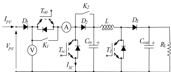
Figure 3. Scheme of the power device
