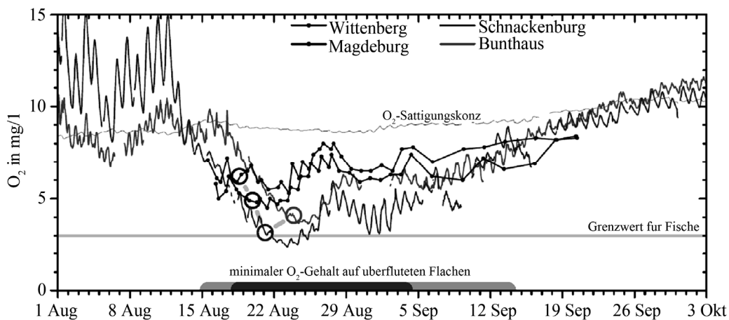
Figure 8. Dissolved oxygen concentrations at Wittenberg, Magdeburg, Schnackenburg and Bunthaus (last three locations ≈ 105, 260 and 390 km downstream from Wittenberg) during the August 2002 flood of the Elbe River, adapted from [13]
