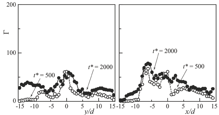
Figure 10. Distribution of \Gamma at density interface ( z/d = 12 ) at Re = 2139 .
