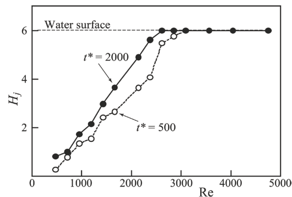
Figure 3. Relationship between Reynolds number Re and nondimensional jet height H_j .
