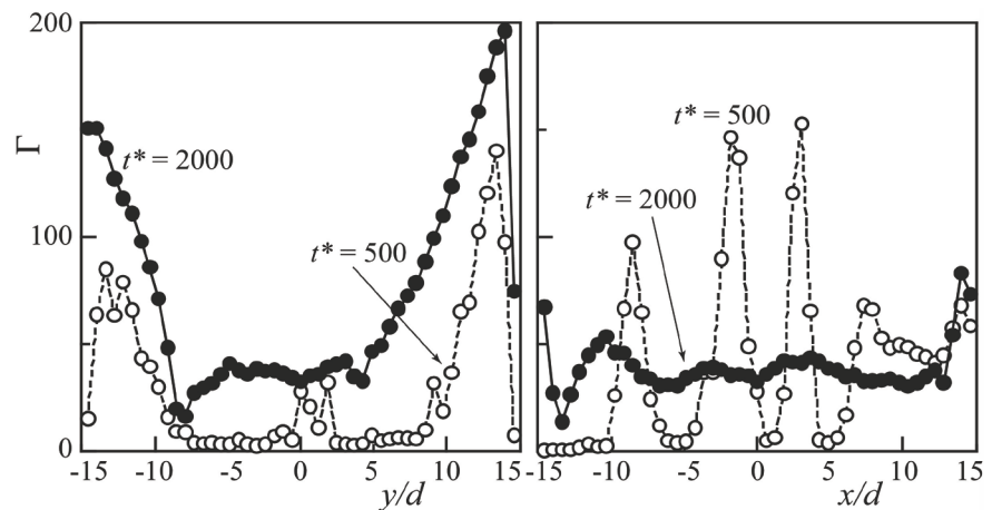
Figure 9. Distribution of \Gamma in lower cross-section ( z/d = 9 ) at Re = 475 .
