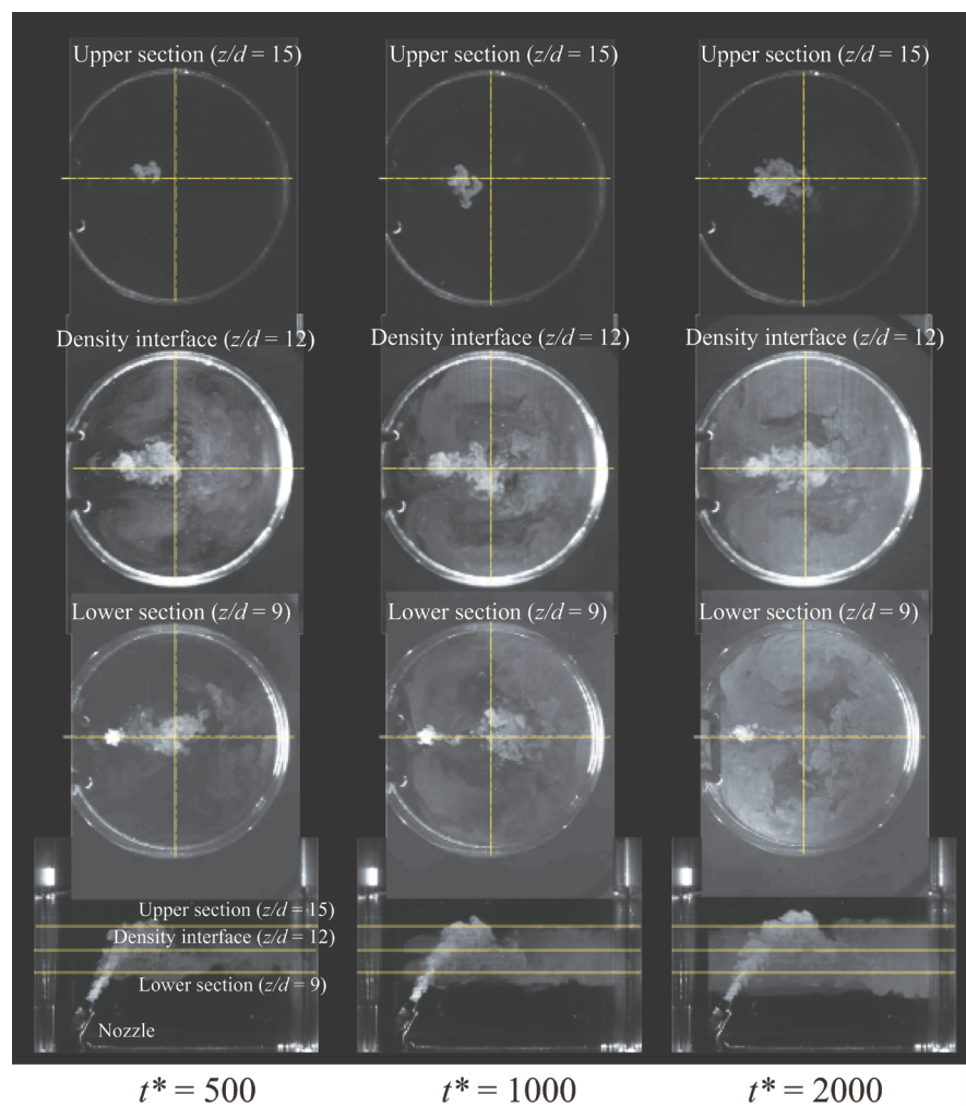
Figure 7. Flow visualized in central vertical and horizontal cross-sections at Re = 2139 .
