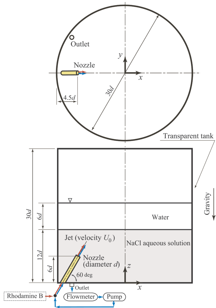
Figure 1. Schematic of experimental setup.
