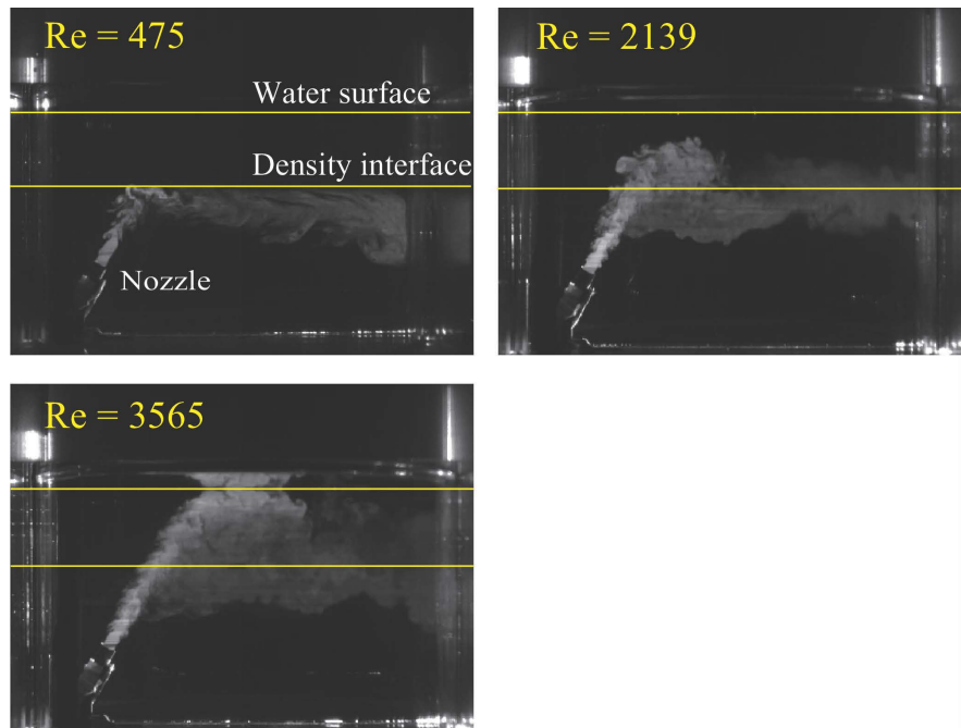
Figure 4. Flow visualized in central vertical cross-section of tank at t' = 500 .
