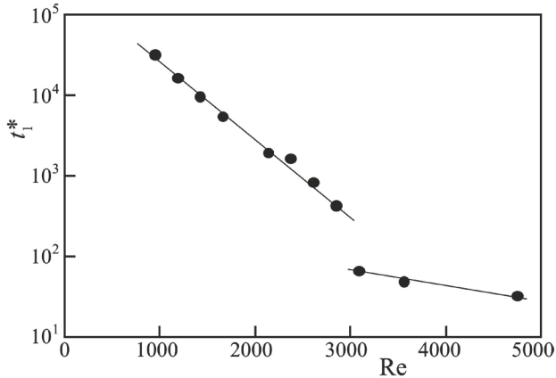
Figure 5. Effect of Re on time of arrival of jet at water surface t_1^* .
