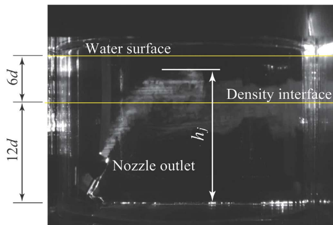
Figure 2. Visual image showing the definition of the jet height h_j .
