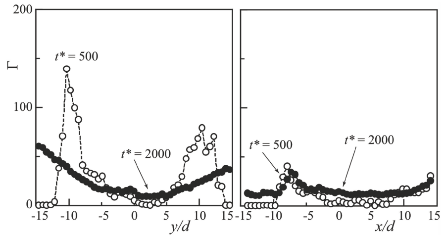
Figure 11. Distribution of \Gamma at density interface ( z/d = 12 ) at Re = 3565 .
