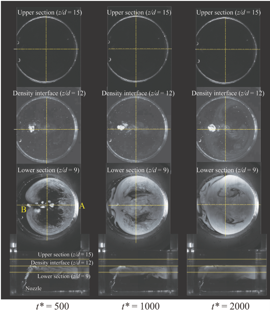
Figure 6. Flow visualized in central vertical and horizontal cross-sections at Re = 475.
