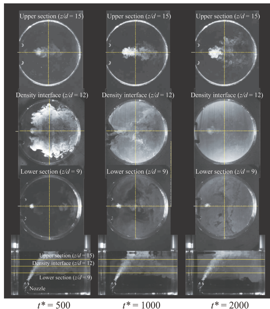
Figure 8. Flow visualized in central vertical and horizontal cross-sections at Re = 3565 .
