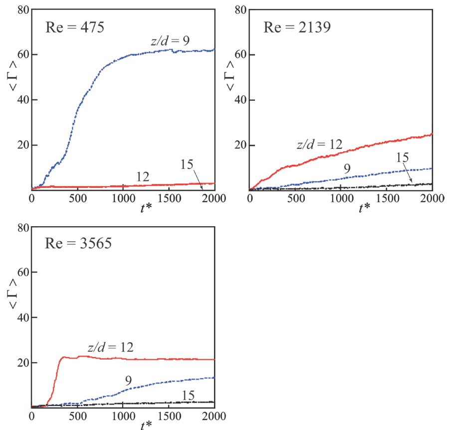
Figure 12. Temporal variation of spatially averaged values of \Gamma at density interface and in horizontal cross-sections.
