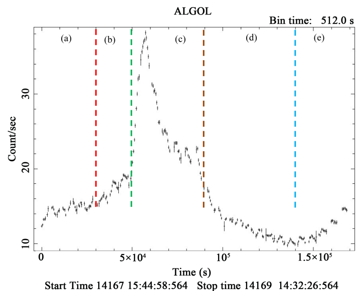
Figure 1. Background subtracted X-ray light-curve of Algol stellar flares.
