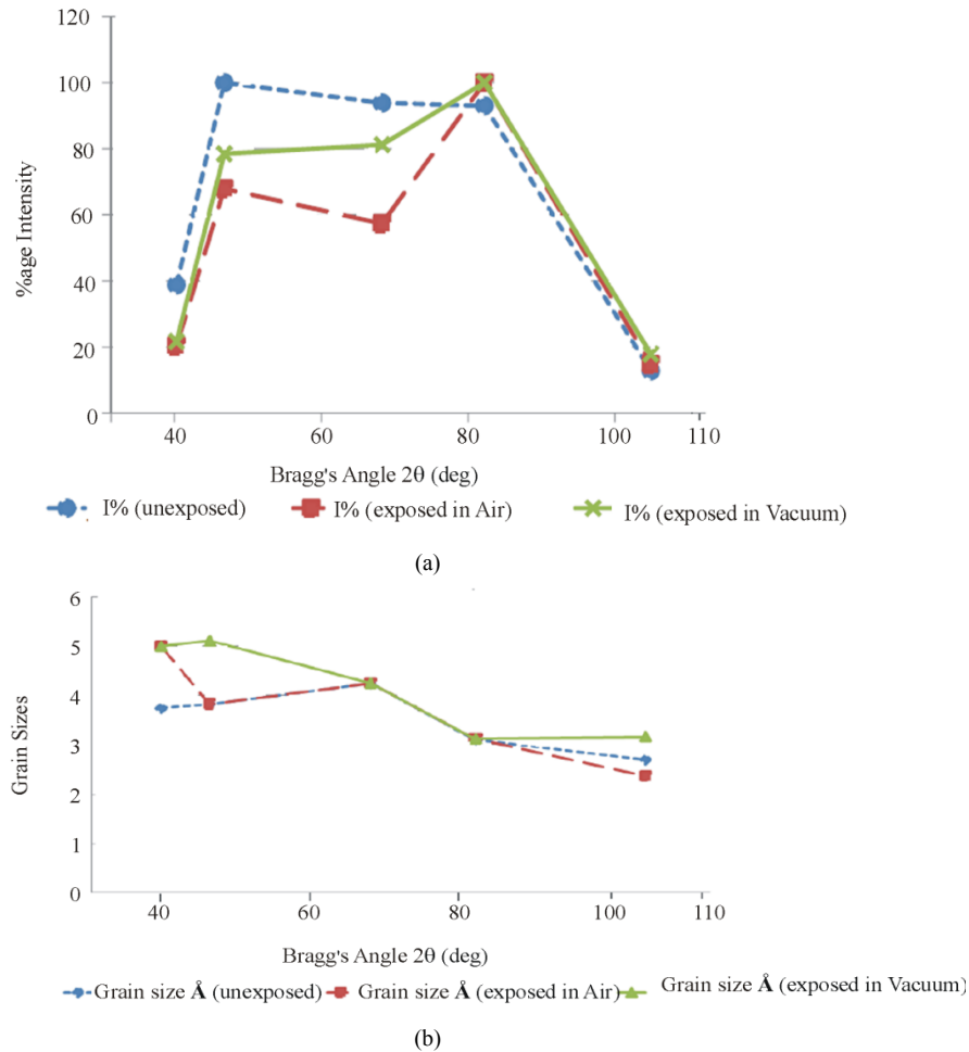
Figure 11. The plots of (a) diffracted X-ray intensity vs. Bragg's angle 2\theta (b) Grain sizes vs. Bragg's angle 2\theta .
