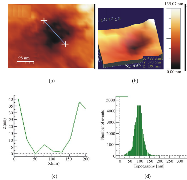
Figure 7. (a) AFM micrograph, crater formation measurement (b) Crater appearing as a part on the Surface (c) Crater size and depth (Size = 180.50 nm, Depth = 40nm) (d) Surface roughness measurement by topographic histogram (rms roughness = 23.91 μm).
