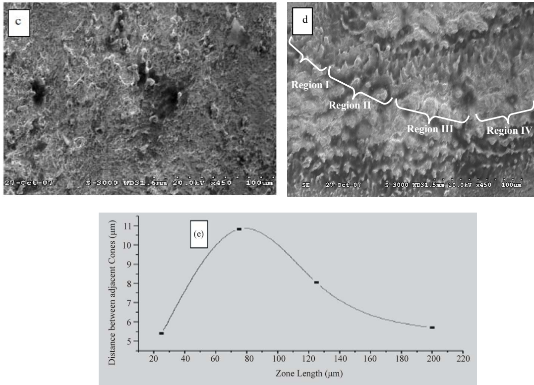
Figure 2. SEM Micrographs of platinum samples (a) ( \times 30 ) irradiated in air for 50 shots. (b) ( \times 180 ) irradiated in air for 50 shots. (c) ( \times 450 ) irradiated in air for 50 shots. (d) ( \times 450 ) irradiated under vacuum ( \sim 10^3 torr) for 50 shots (e) Plot of average zone length ( \mu\text{m} ) versus the distance between adjacent cones ( \mu\text{m} ).
