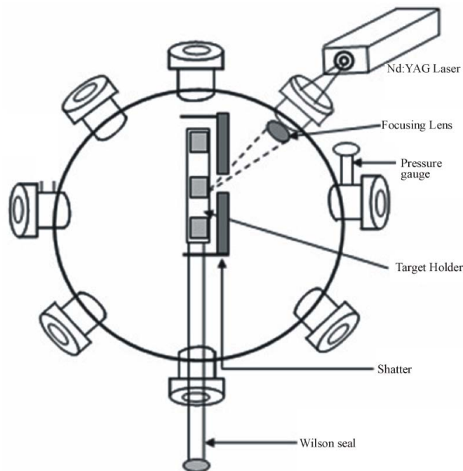
Figure 1. A Schematic of the Experimental set up.
