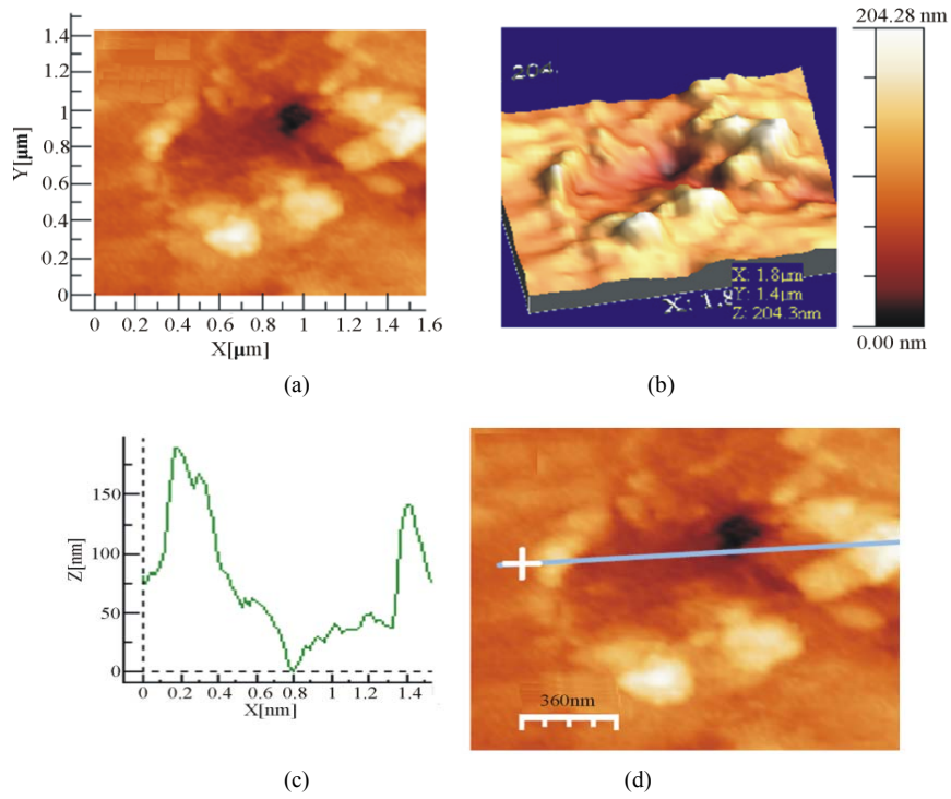
Figure 6. AFM micrographs (a) indicating crater formation due to laser irradiation (b) showing a valley, craters surrounded by various hills on the target surface (c) Surface profile of the formed valley (d) Average size measurement of the valley (1.50 μm).
