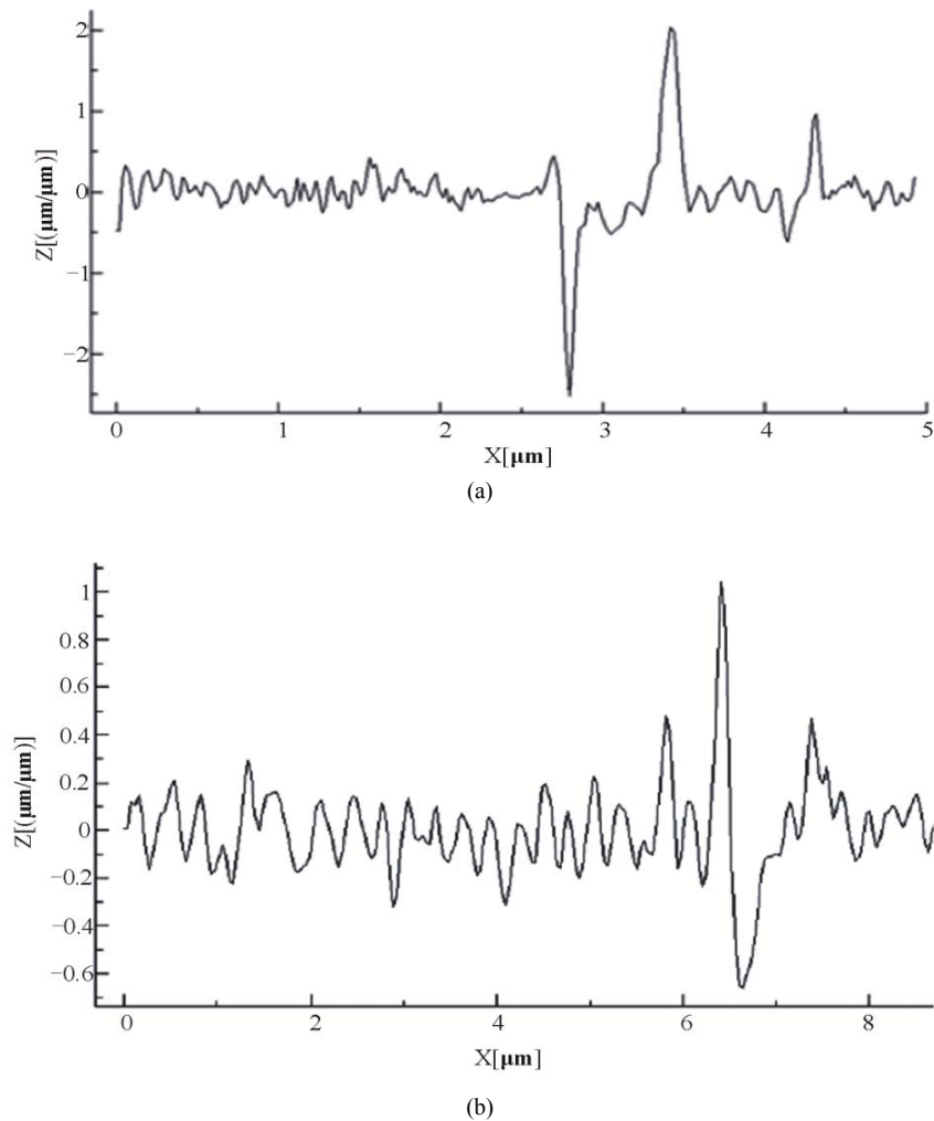
Figure 4. Surface profile (a) irradiated target in air (b) irradiated target under vacuum ( 10^{-3} torr).
