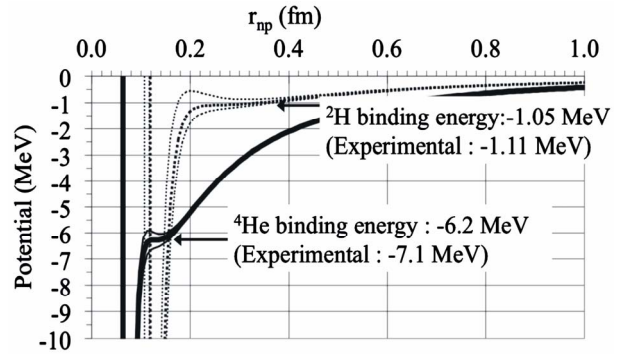
Figure 4. ^2\text{H} and ^4\text{He} electromagnetic energy potentials per nucleon from Formulas (22) and (28). The binding energies are obtained graphically by trial and error from the electric and magnetic Coulomb's potentials by varying the neutron proton distance r_{np} and the dipole separation 2a until a relative minimum is obtained, unfortunately a flat spot, due to the Coulomb singularity. A true minimum was obtained for the deuteron when the positive charge of the neutron is neglected [10]. Only fundamental constants are used, no fitting or ad hoc parameters.
