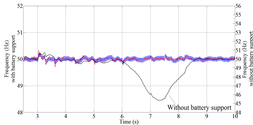
Figure 8. Frequency profiles.
