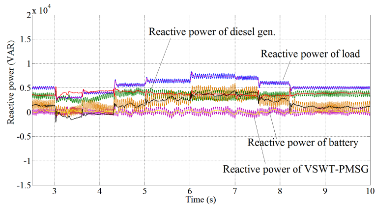
Figure 6. Reactive power profiles.
