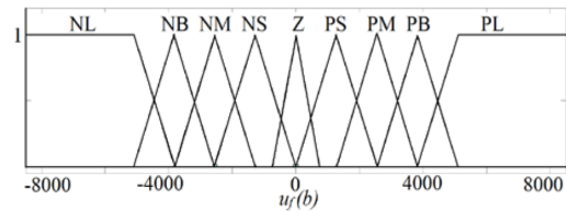
(b). MFs of FLC f output
