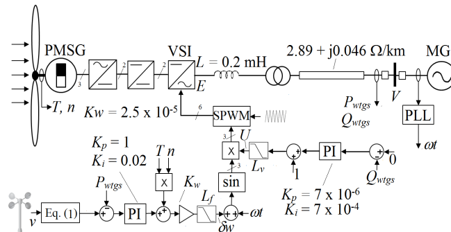
Figure 3. VSWT-PMSG inverter controller.
