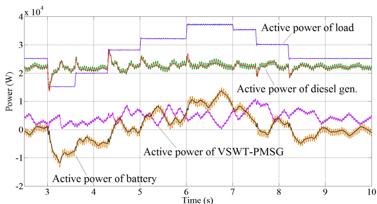
Figure 5. Active power profiles.
