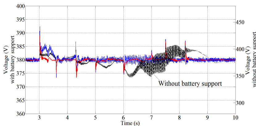
Figure 9. Voltage profiles.
