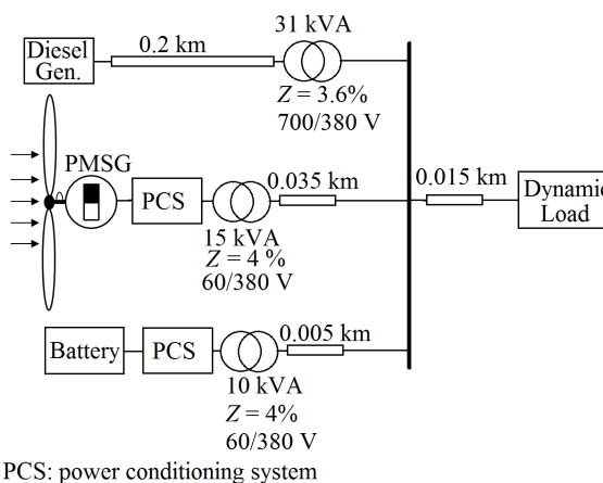
Figure 1. Isolated MG with embedded small VSWT-PMSG and batteries.
