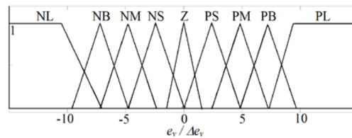
(c). MFs of FLC v input
