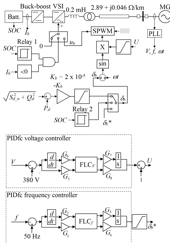
Figure 4. Battery inverter controller.
