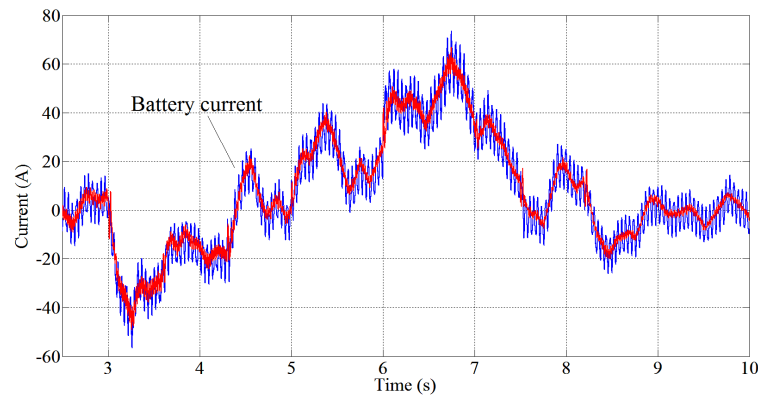
Figure 7. Battery current profiles.
