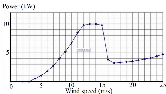
Figure 2. Alize Fortis wind turbine characteristics.
