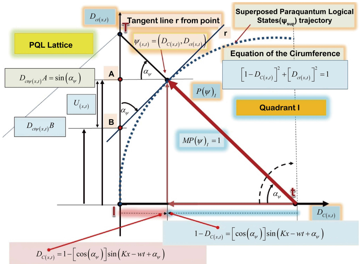
Figure 4. Tangent line r at the point where the Paraquantum logical state is located on the vertex of State Vector P(\psi)_I , where it meets B , on the contradiction degree axis.
