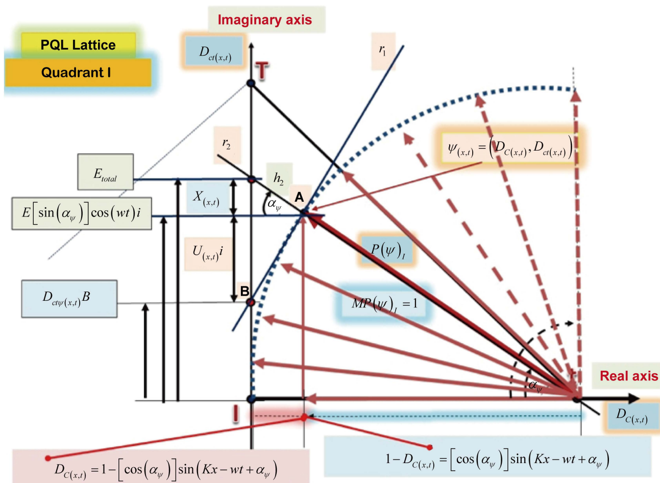
Figure 6. Representation of energy function values related to a time-dependent Schrödinger's equation along the axis of the contradiction degrees.
