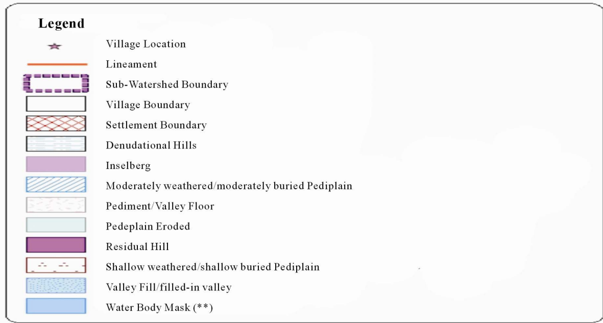
Figure 2. Water bodies and lineaments.
