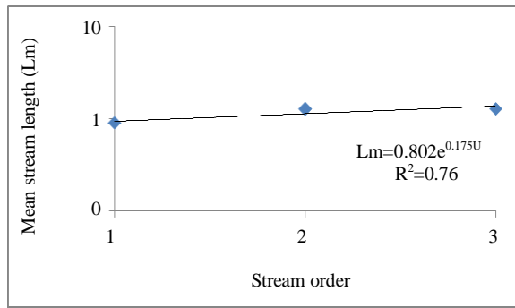
Figure 3. Regression of log. of mean stream length V/s stream order.
