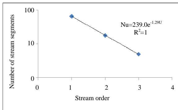
Figure 4. Regression of log. of number stream segments/s stream order.
