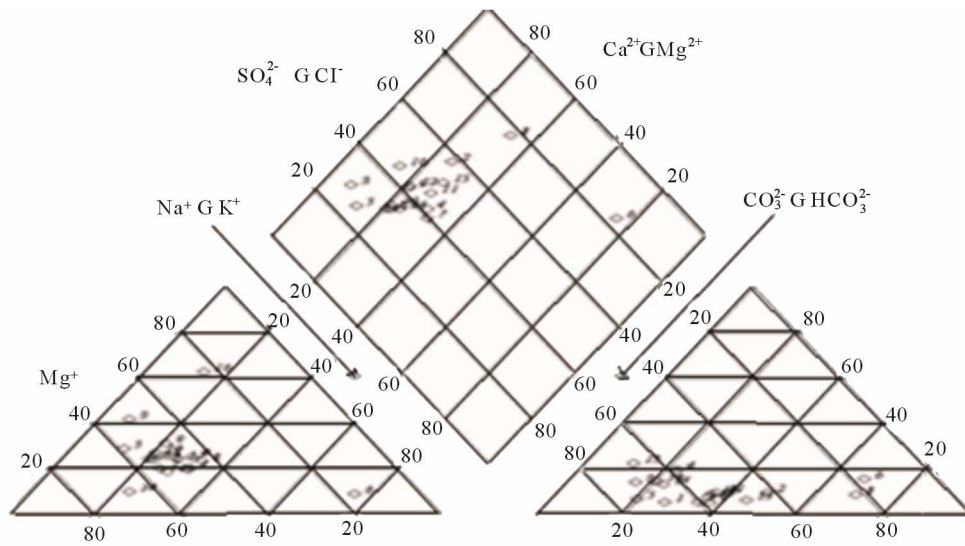
Figure 5. Piper tri-linear diagram showing the chemical composition of ground water during post monsoon.
