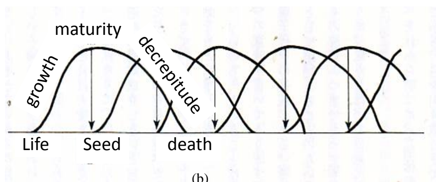
Figure 5. Metaphorical expression for Irradiated frequencies and waves of life [43] [44]. (a) Irradiated frequencies; (b) Waves of life.
