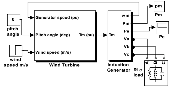
Figure 9. Wind generation system model.
