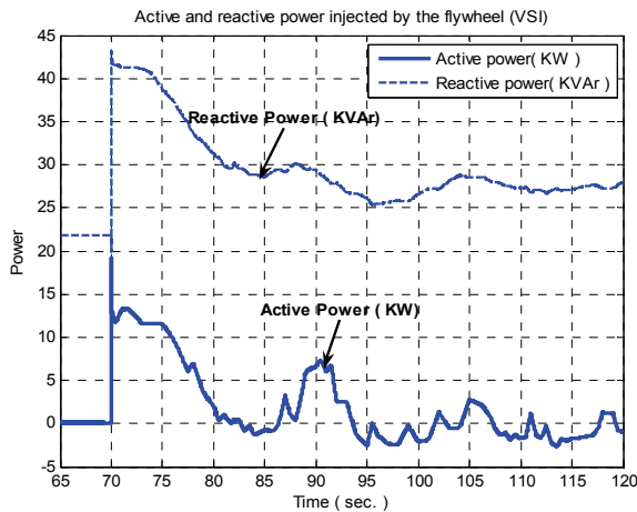
Figure 21. Flywheel ( Vf inverter) active and reactive powers.
