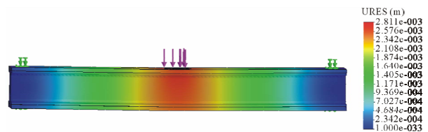
Figure 6. Three points loading beam finite element analysis results.
