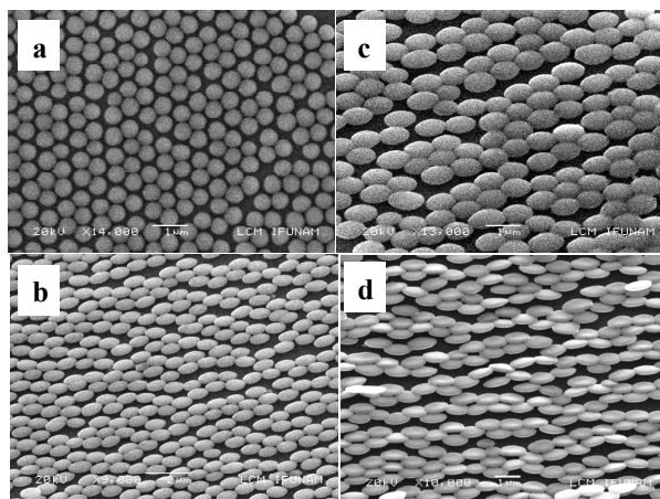
Figure 2. SEM micrographs corresponding to: (a) As-prepared spherical silica particles (top view); (b) 1.5 \times 10^{15} \text{Si}/\text{cm}^2 , (c) 3 \times 10^{15} \text{Si}/\text{cm}^2 , (d) 4.5 \times 10^{15} \text{Si}/\text{cm}^2 irradiated samples (viewed in a direction perpendicular to the irradiation beam, under an angle of 45^\circ with respect to the sample surface). The scale bar is 1 \mu\text{m} , except for (b), where it corresponds to 2 \mu\text{m} .
