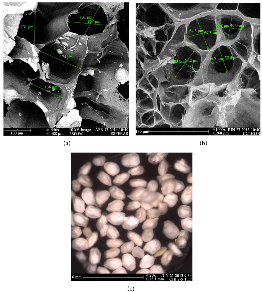
Figure 1. SEM of chitosan scaffolds microstructure (a) 550 \times ; (b) 1000 \times and (c) 2000 \times .
